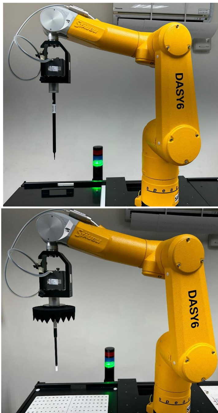
Fig.1 Photograph of the SAR measurement system
