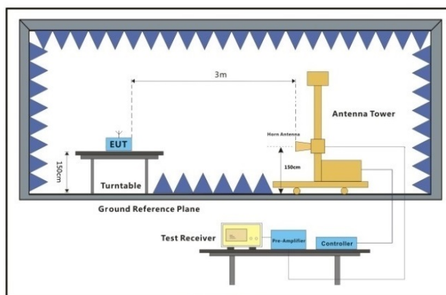
Above 1GHz
