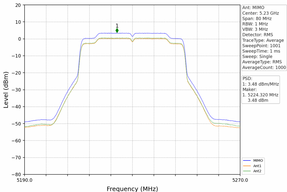
802.11ax(HEW40)_HCH_5230MHz_RU484_Left_MIMO_NTNV
