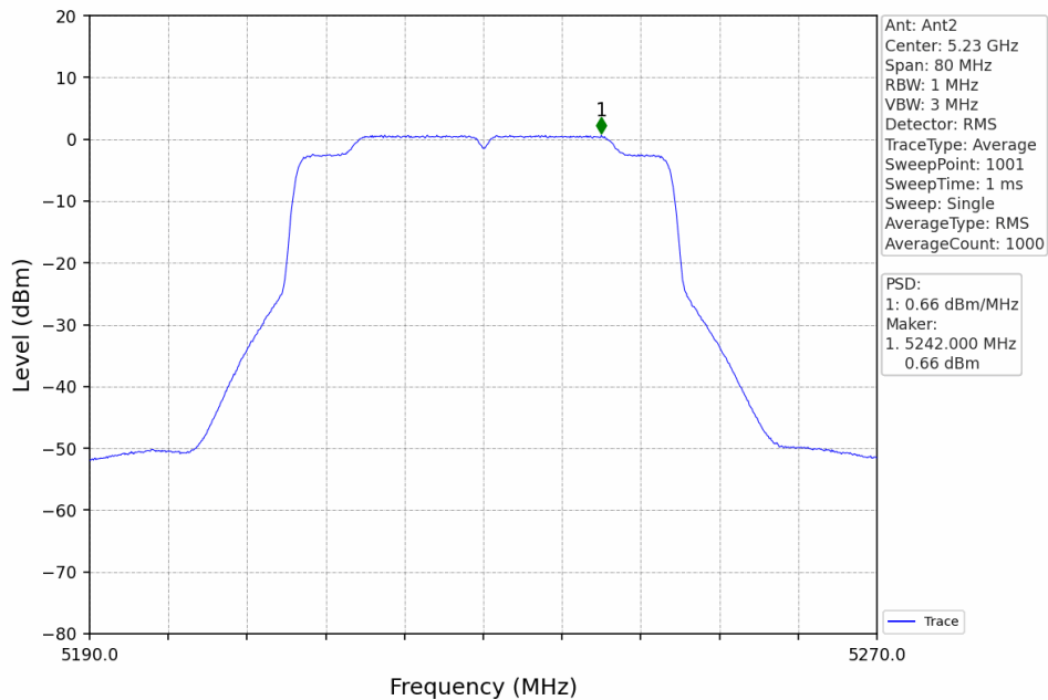
802.11ax(HEW40)_HCH_5230MHz_RU484_Left_MIMO_NTNV
