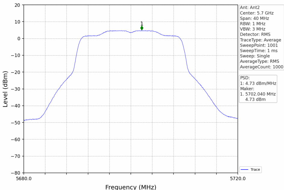
802.11ax(HEW20)_HCH_5700MHz_RU242_Left_MIMO_NTNV
