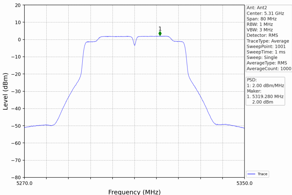
802.11ac(VHT40)_HCH_5310MHz_MIMO_NTNV
