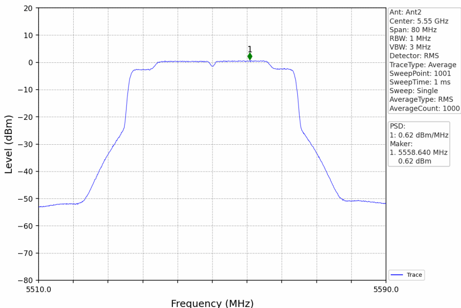
802.11ax(HEW40)_MCH_5550MHz_RU484_Left_MIMO_NTNV
