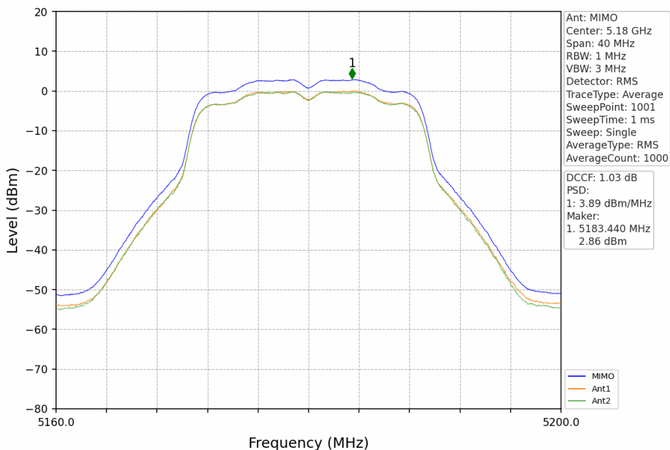
802.11ac(VHT20)_LCH_5180MHz_MIMO_NTNV
