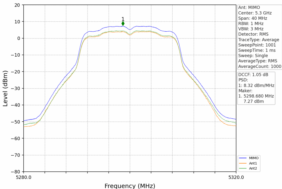
802.11ac(VHT20)_MCH_5300MHz_MIMO_NTNV
