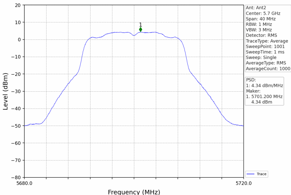
802.11ac(VHT20)_HCH_5700MHz_MIMO_NTNV
