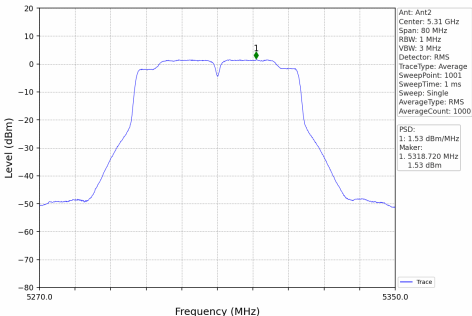
802.11n(HT40)_HCH_5310MHz_MIMO_NTNV
