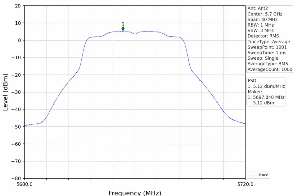
802.11n(HT20)_HCH_5700MHz_MIMO_NTNV
