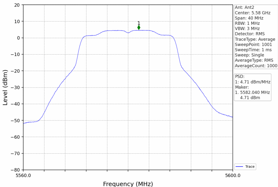
802.11n(HT20)_MCH_5580MHz_Ant2_NTNV
