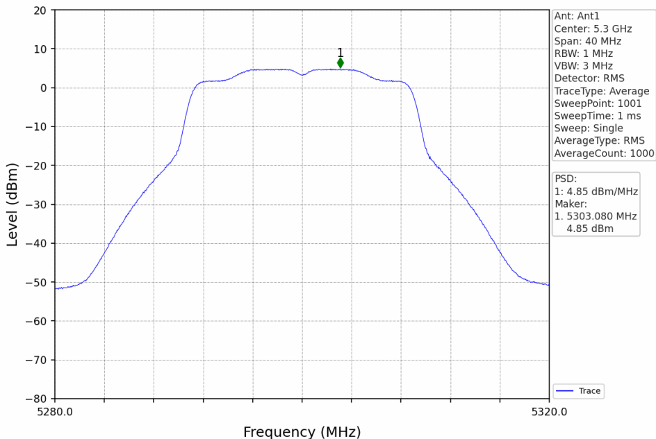
802.11n(HT20)_MCH_5300MHz_Ant1_NTNV
