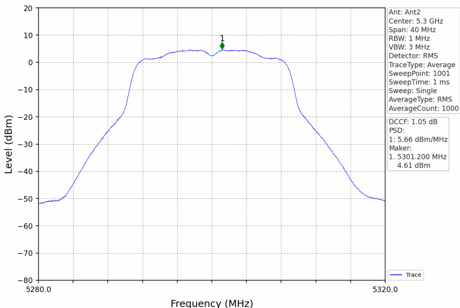
802.11ac(VHT20)_MCH_5300MHz_MIMO_NTNV
