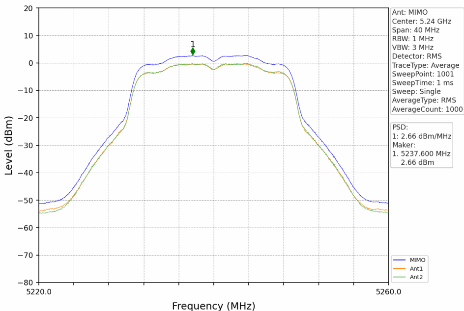
802.11ac(VHT20)_HCH_5240MHz_MIMO_NTNV
