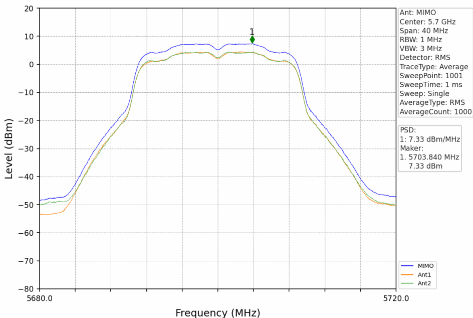
802.11ac(VHT20)_HCH_5700MHz_MIMO_NTNV
