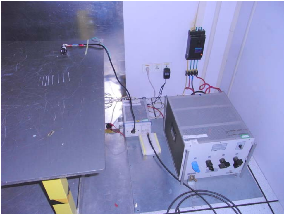
Line Conducted Emission Test Setup
