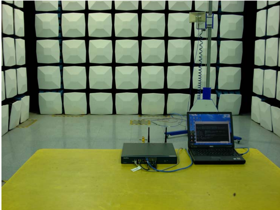
Radiated Spurious Emission Test Setup Rear View (Above 1 GHz)
