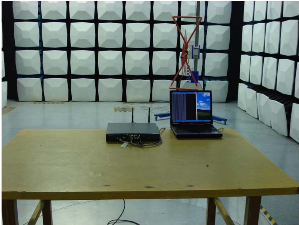
Radiated Spurious Emission Test Setup Rear View (Blow 1 GHz)
