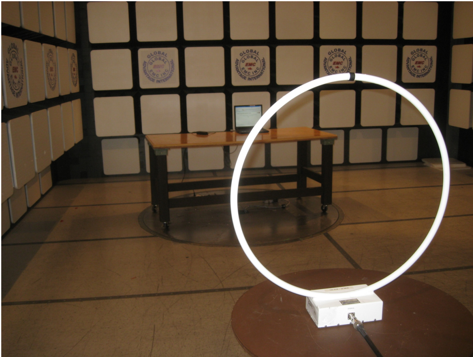
Radiated Emissions – Loop
