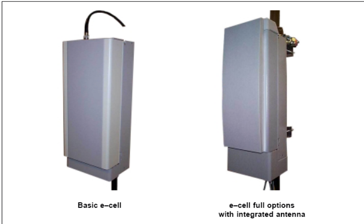
Figure 1-1 BTS overview
