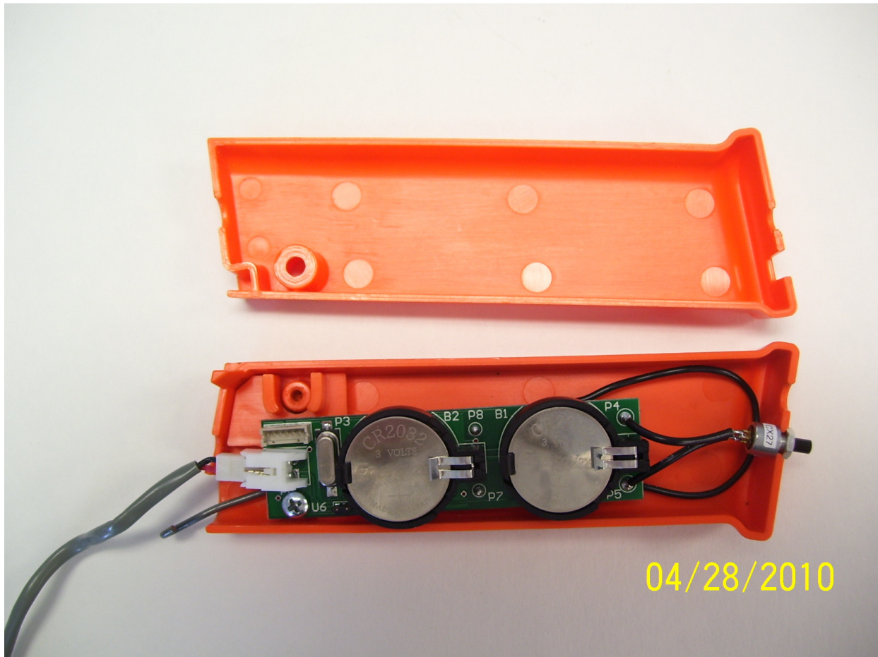
RS-MGZ Plastic Enclosure
