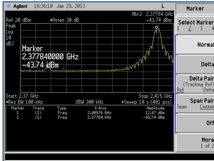
FIGURE 13 - LOWER BANDEGE (2370-2415)
