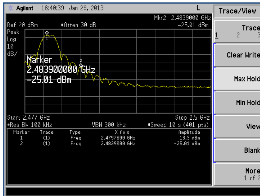
FIGURE 14 - UPPER BANDEGE (2477 - 2500)
