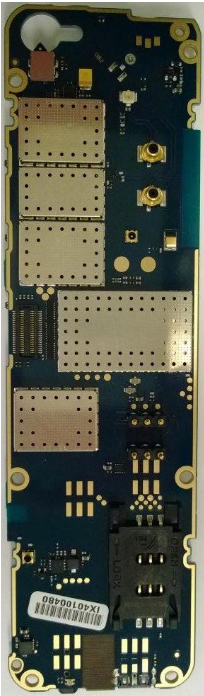
PWB Bottom side, with shields
