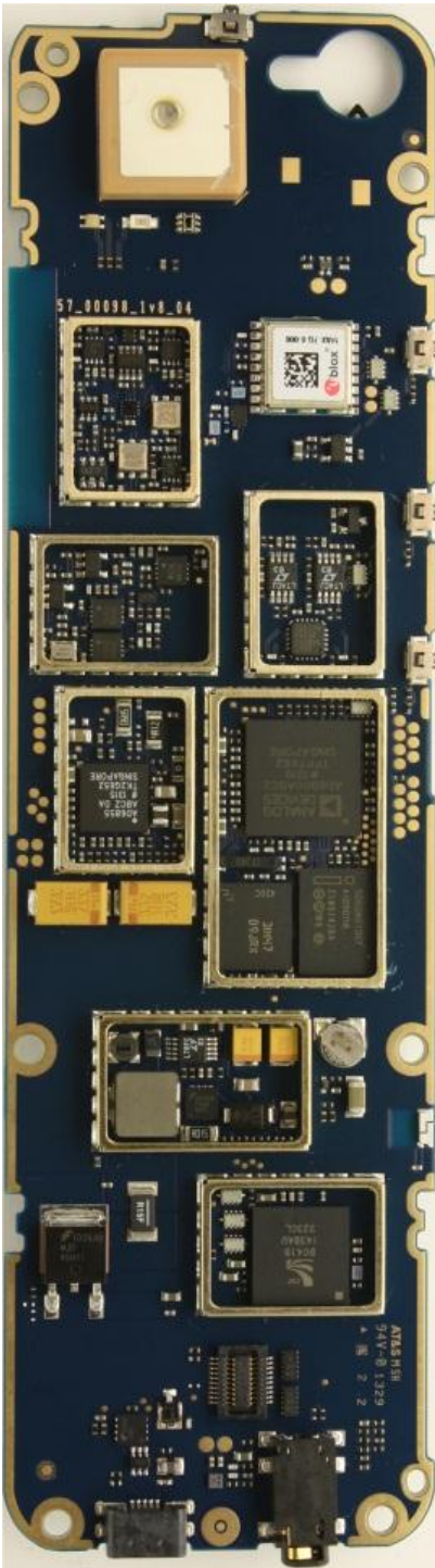
PWB Top side, without shield tops
