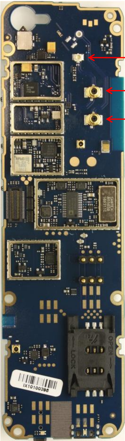
PWB Bottom side, without shield tops
