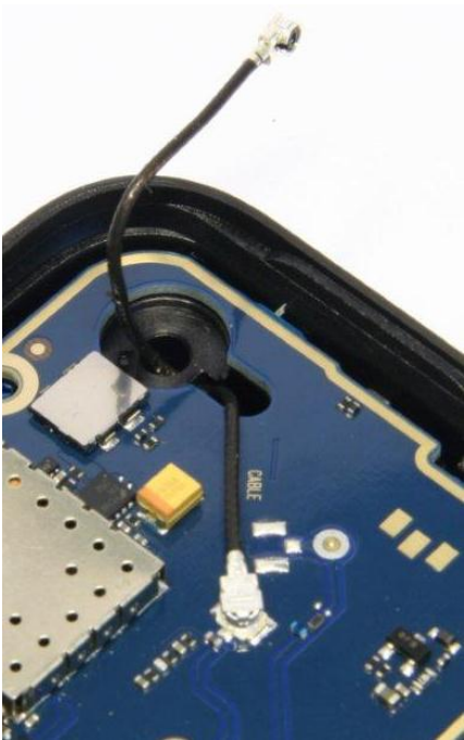
Antenna Cable
