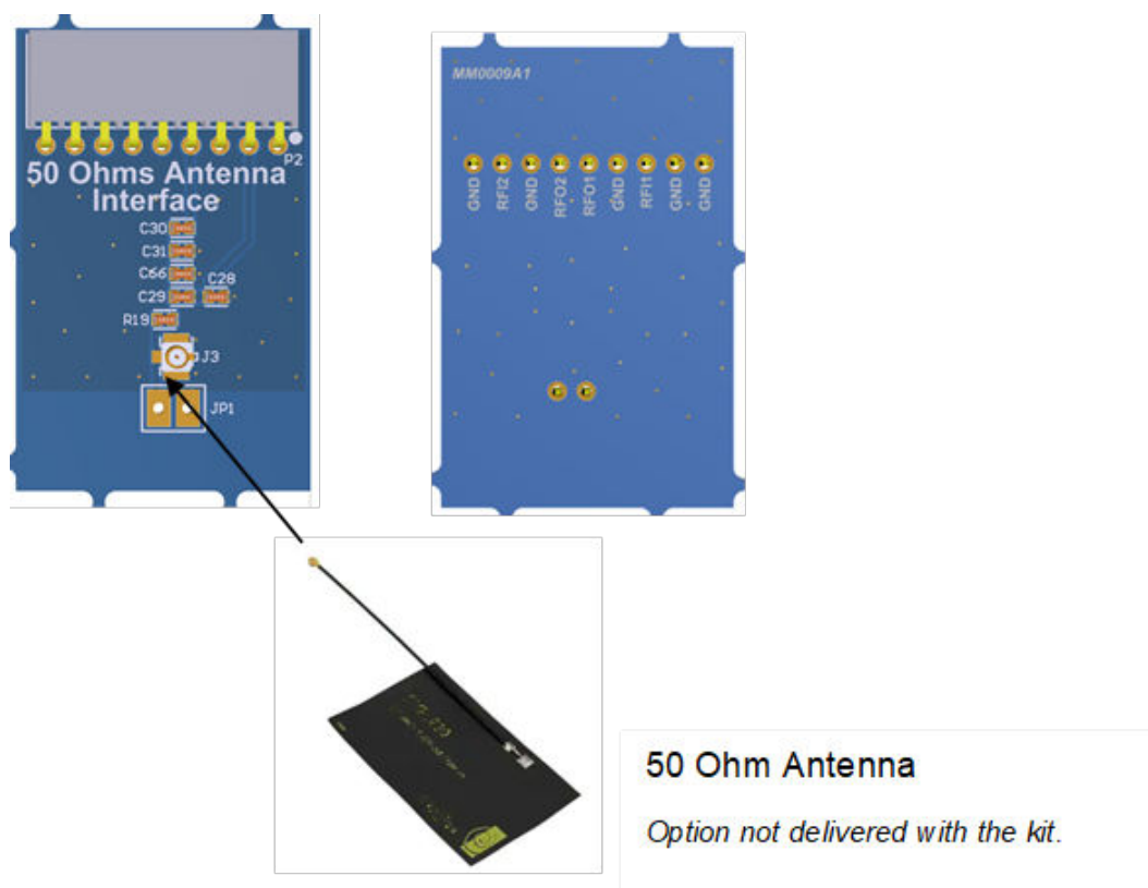
Figure 12. 50-ohm antenna
