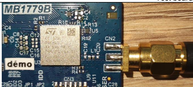
Test board detailed view
