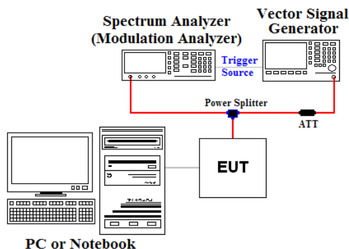
WiMAX Conducted Power Test Setup Diagram
