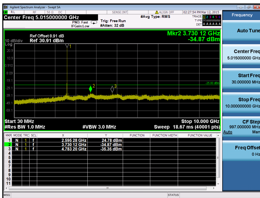
LTE Band 41 / 5MHz / 16QAM - RB Size/Offset (1/24) – Mid Channel
