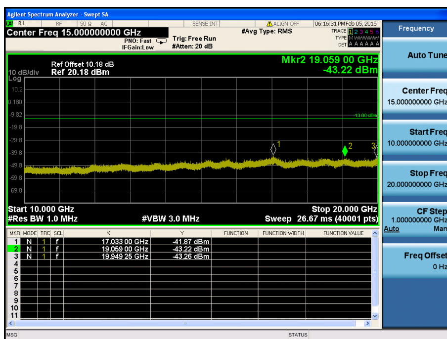
LTE Band 25 / 15MHz / QPSK - RB Size/Offset (1/0) – Mid Channel
