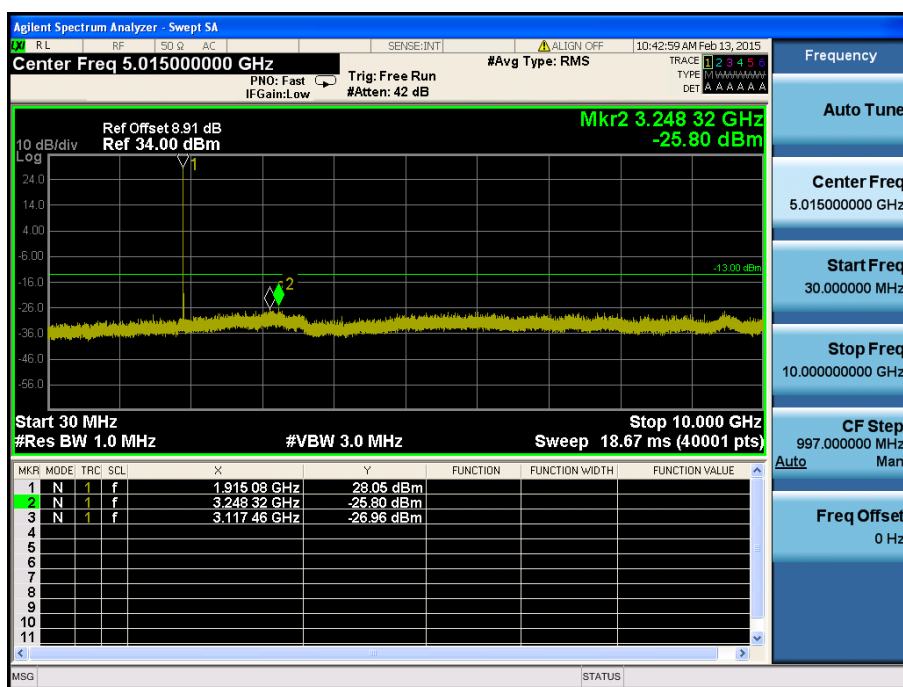
LTE Band 25 / 3MHz / QPSK - RB Size/Offset (1/14) – High Channel
