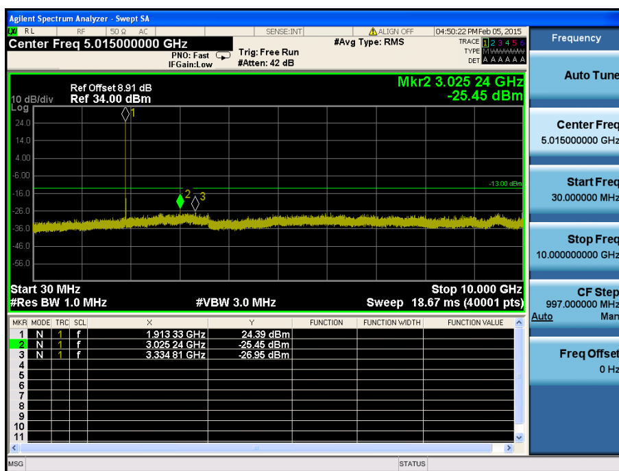
LTE Band 25 / 5MHz / QPSK - RB Size/Offset (12/13) – High Channel
