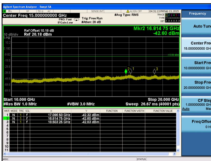
LTE Band 25 / 1.4MHz / 16QAM - RB Size/Offset (3/0) – Mid Channel
