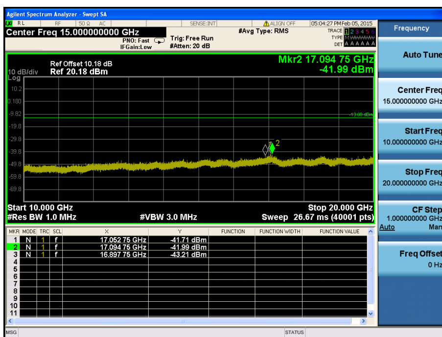
LTE Band 25 / 10MHz / QPSK - RB Size/Offset (1/49) – Low Channel
