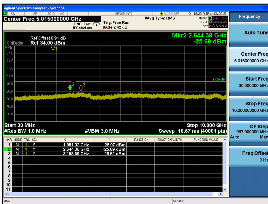
LTE Band 25 / 1.4MHz / 16QAM - RB Size/Offset (3/1) – Low Channel
