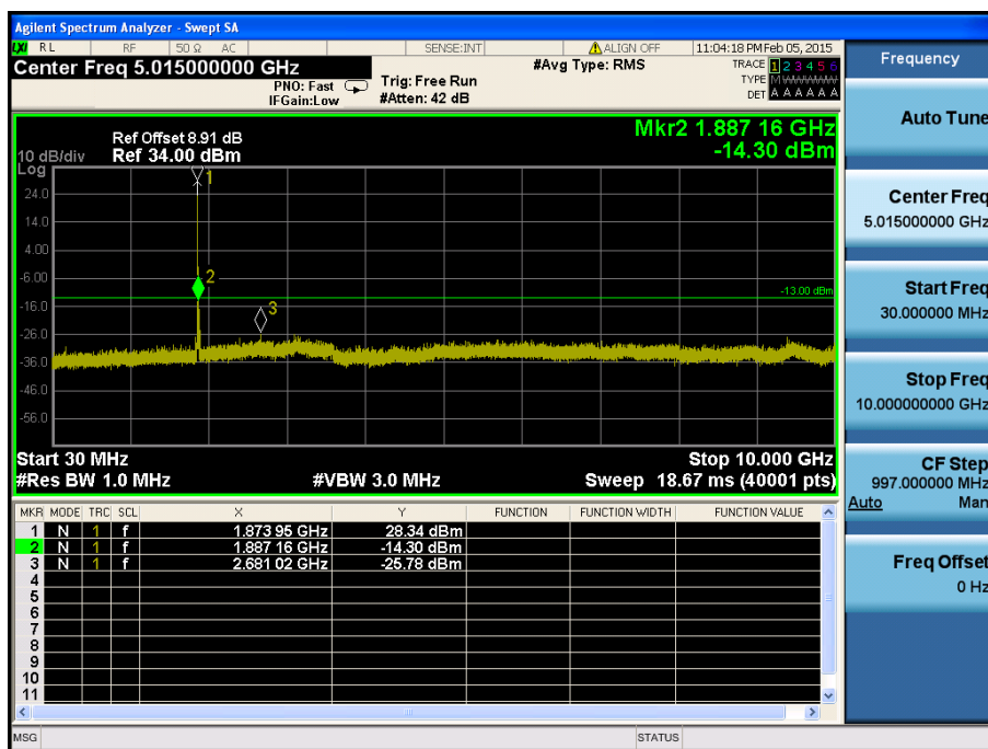
LTE Band 25 / 20MHz / 16QAM - RB Size/Offset (1/0)–Mid Channel
