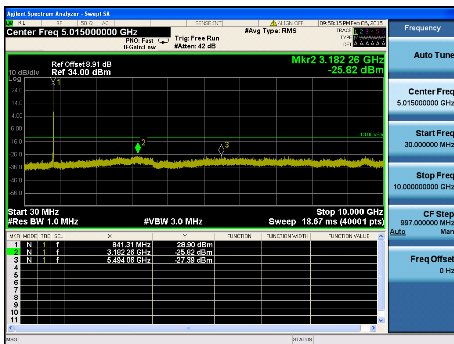
LTE Band 26 / 10MHz / QPSK - RB Size/Offset (1/49) – Mid Channel
