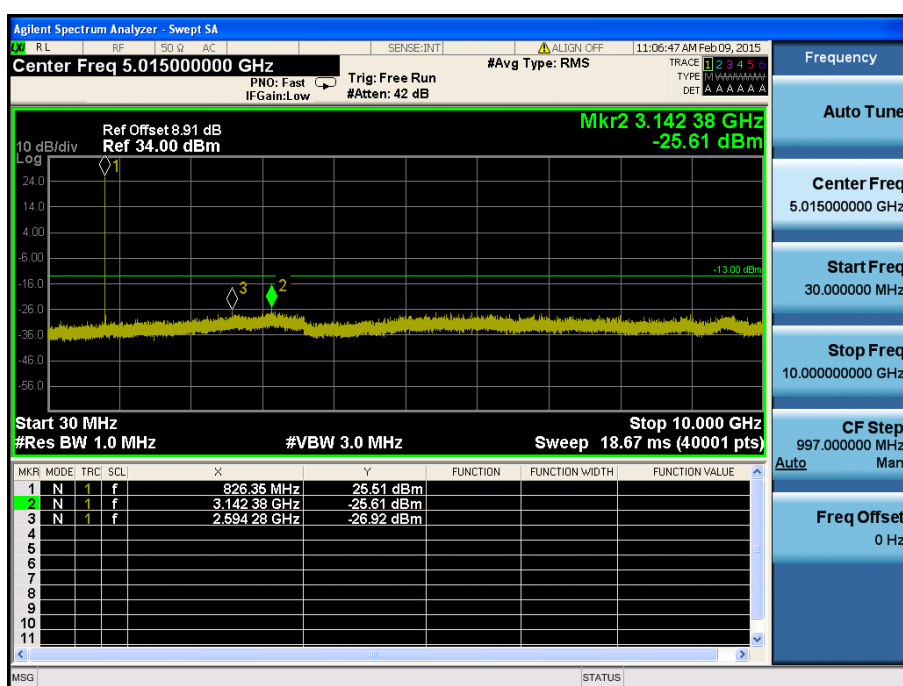
LTE Band 26 / 3MHz / 16QAM - RB Size/Offset (8/7) – Low Channel
