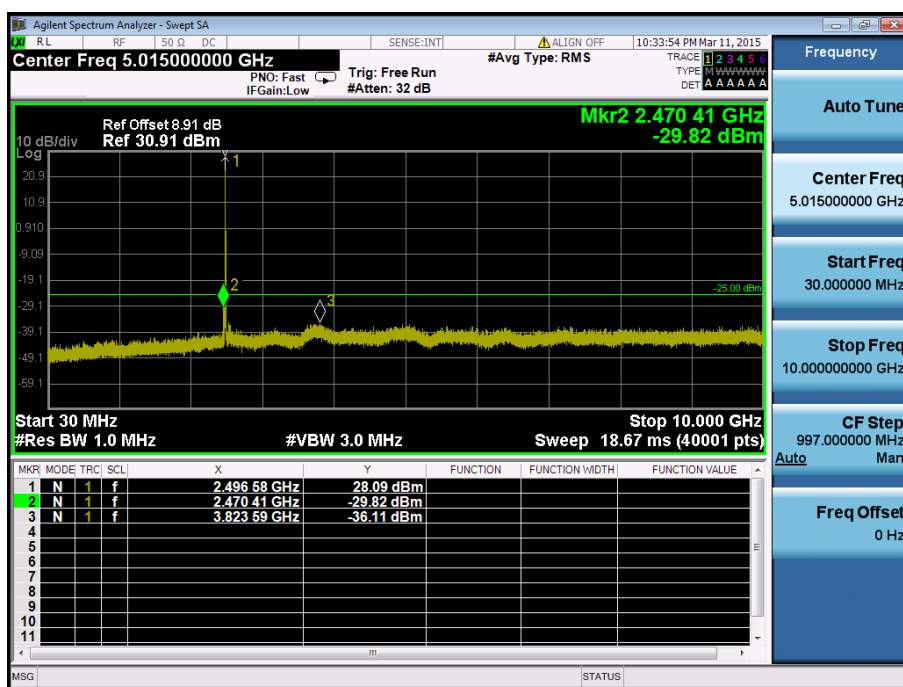
LTE Band 41 / 10MHz / QPSK - RB Size/Offset (1/0) – Low Channel
