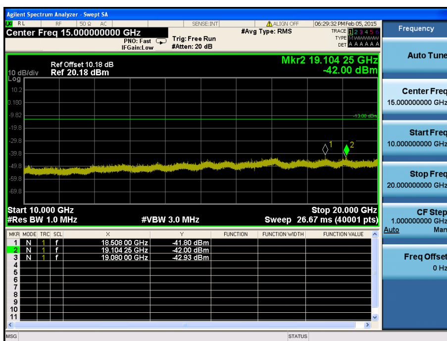
LTE Band 25 / 15MHz / QPSK - RB Size/Offset (1/37) – High Channel
