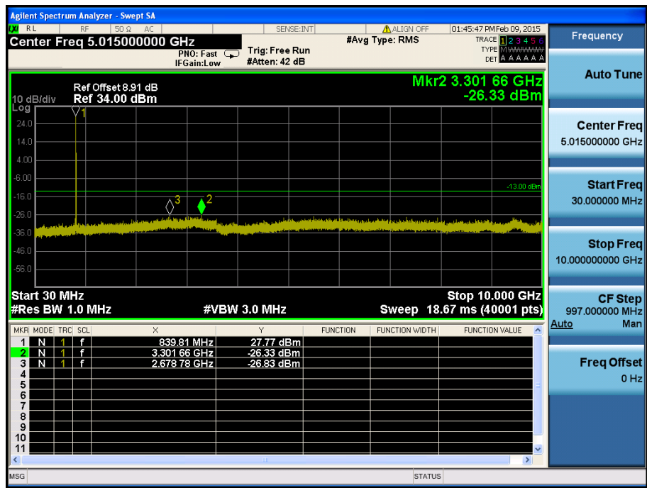
TE Band 26 / 10MHz / 16QAM - RB Size/Offset (1/0) – High Channel
