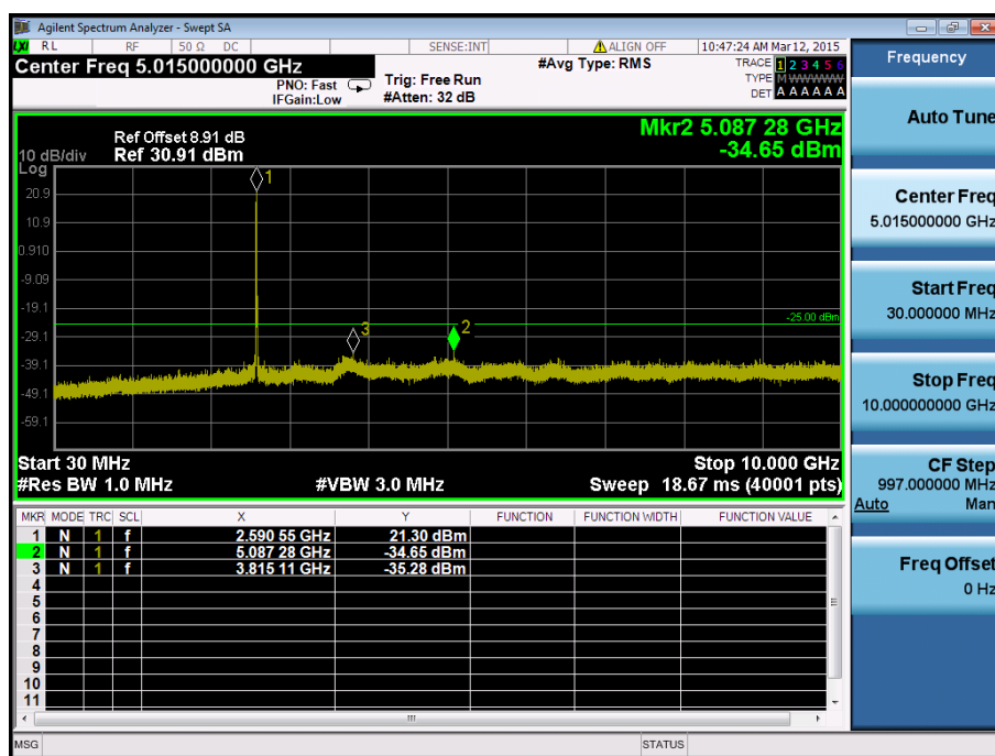
LTE Band 41 / 20MHz / QPSK - RB Size/Offset (50/25) – Mid Channel
