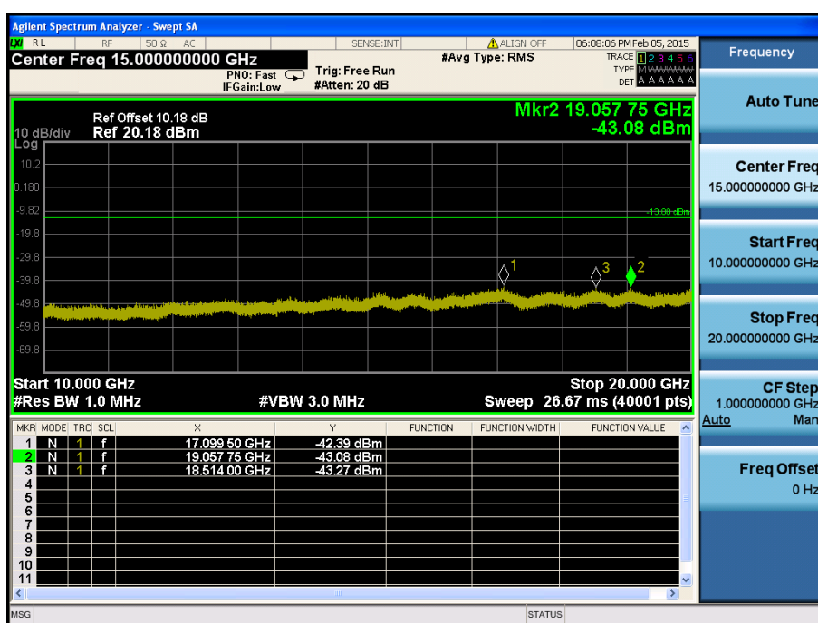
LTE Band 25 / 15MHz / QPSK - RB Size/Offset (36/19)-Low Channel
