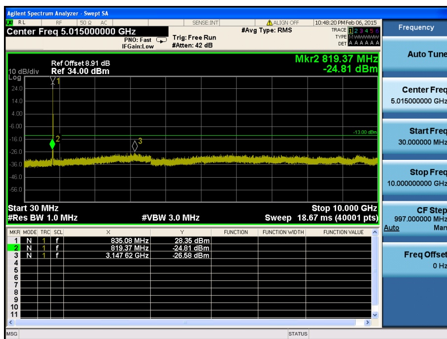
LTE Band 26 / 15MHz / QPSK - RB Size/Offset (1/0) – High Channel
