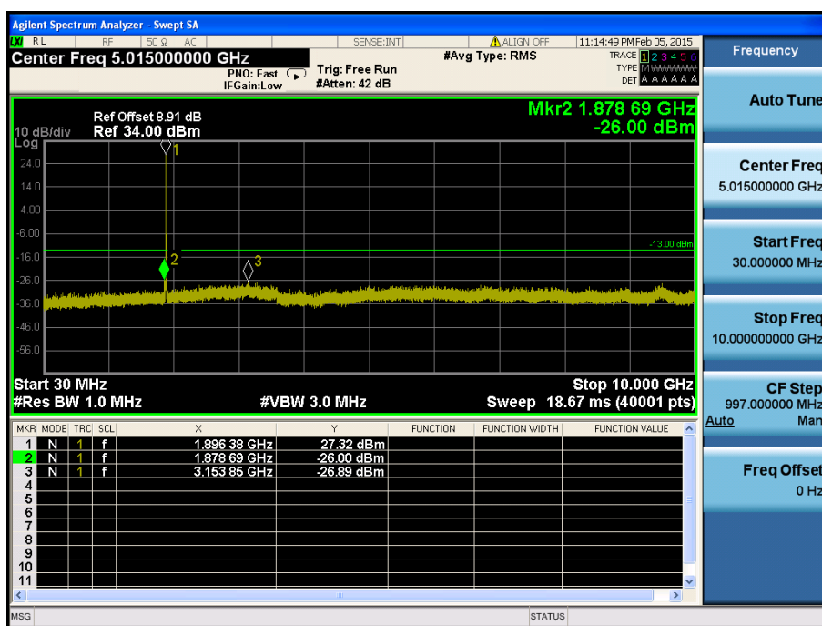
LTE Band 25 / 20MHz / 16QAM - RB Size/Offset (1/0) – High Channel
