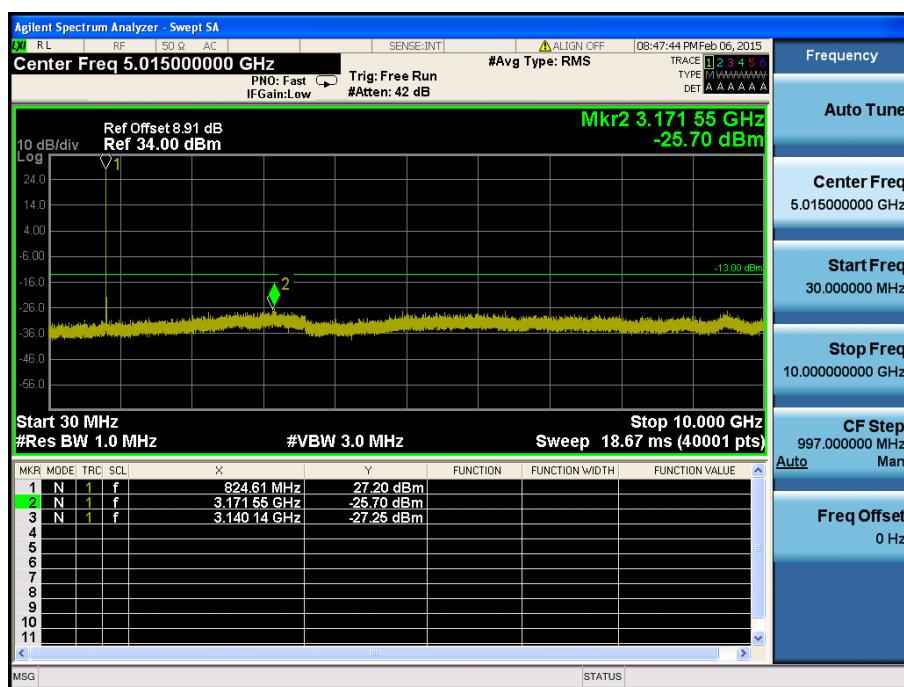
LTE Band 26 / 5MHz / QPSK - RB Size/Offset (1/0) – Low Channel
