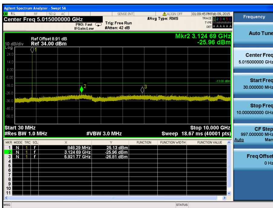
LTE Band 26 / 5MHz / 16QAM - RB Size/Offset (12/13) – High Channel
