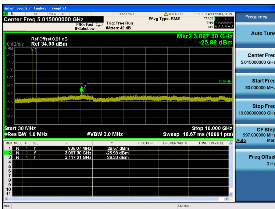
LTE Band 26 / 3MHz / QPSK - RB Size/Offset (1/14) – Mid Channel
