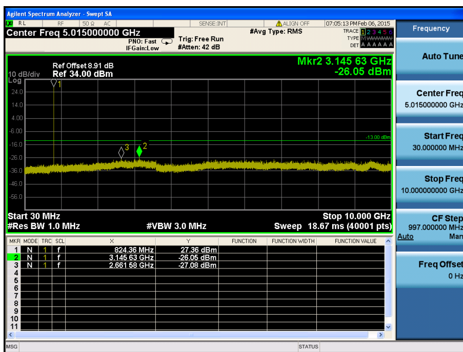
LTE Band 26 / 1.4MHz / QPSK - RB Size/Offset (1/0) – Low Channel
