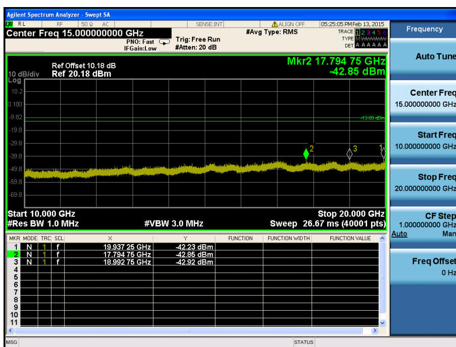
LTE Band 25 / 3MHz / 16QAM - RB Size/Offset (1/0) – Mid Channel
