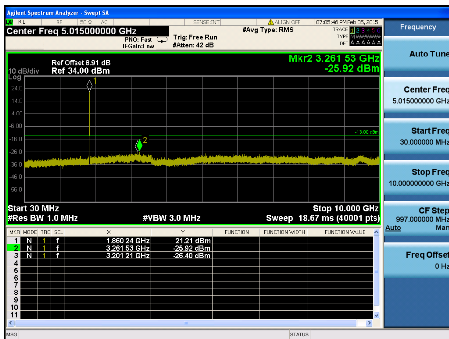
LTE Band 25 / 20MHz / QPSK - RB Size/Offset (50/25) –Low Channel
