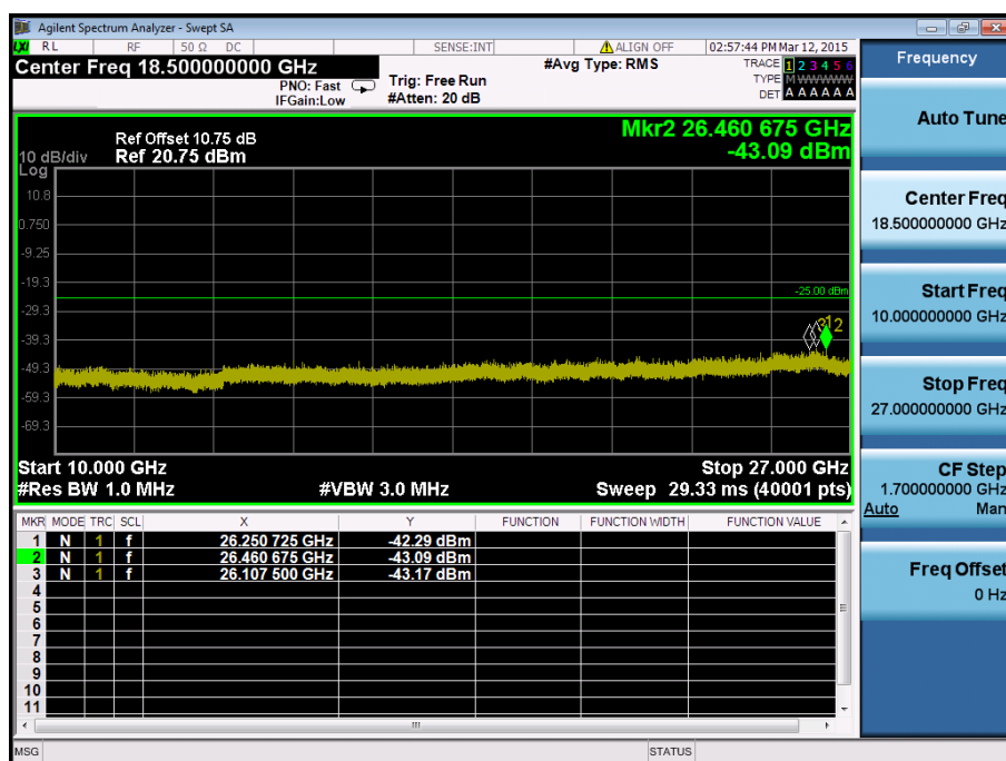
LTE Band 41 / 10MHz / 16QAM - RB Size/Offset (1/0) – Mid Channel
