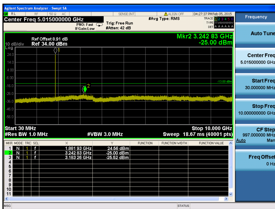
LTE Band 25 / 5MHz / QPSK - RB Size/Offset (12/0) – Mid Channel
