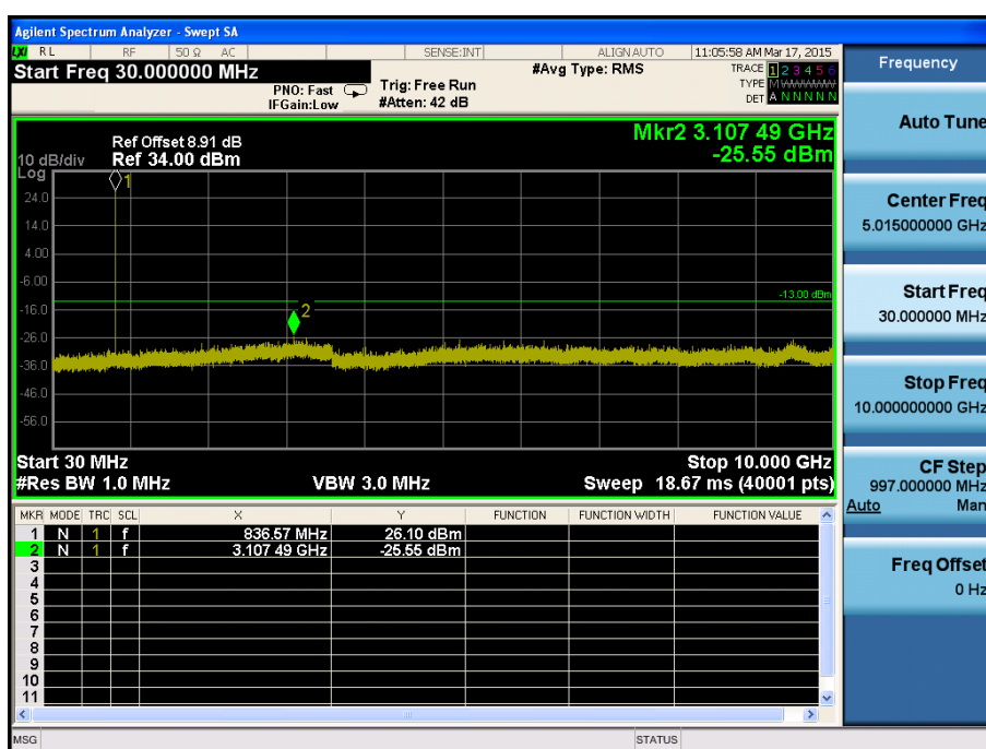
LTE Band 26 / 1.4MHz / QPSK - RB Size/Offset (6/0) – Mid Channel
