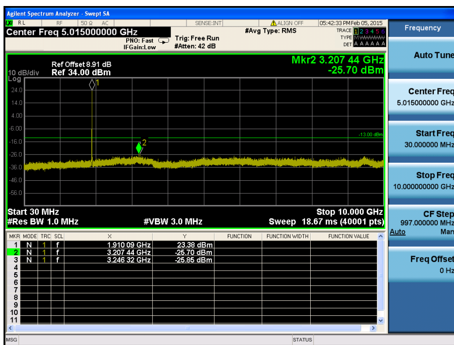
LTE Band 25 / 10MHz / QPSK - RB Size/Offset (25/12) – High Channel
