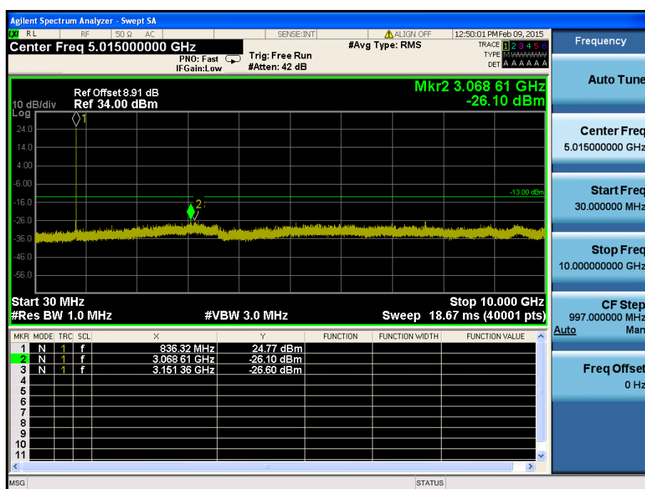
LTE Band 26 / 5MHz / 16QAM - RB Size/Offset (12/0) – Mid Channel
