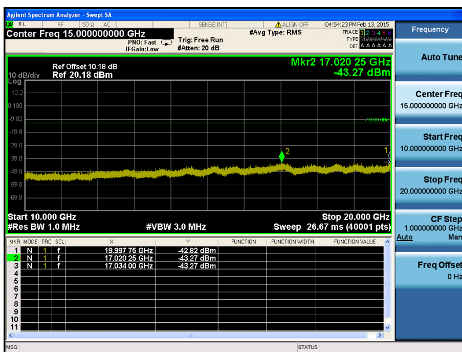
LTE Band 25 / 1.4MHz / 16QAM - RB Size/Offset (3/3) – High Channel
