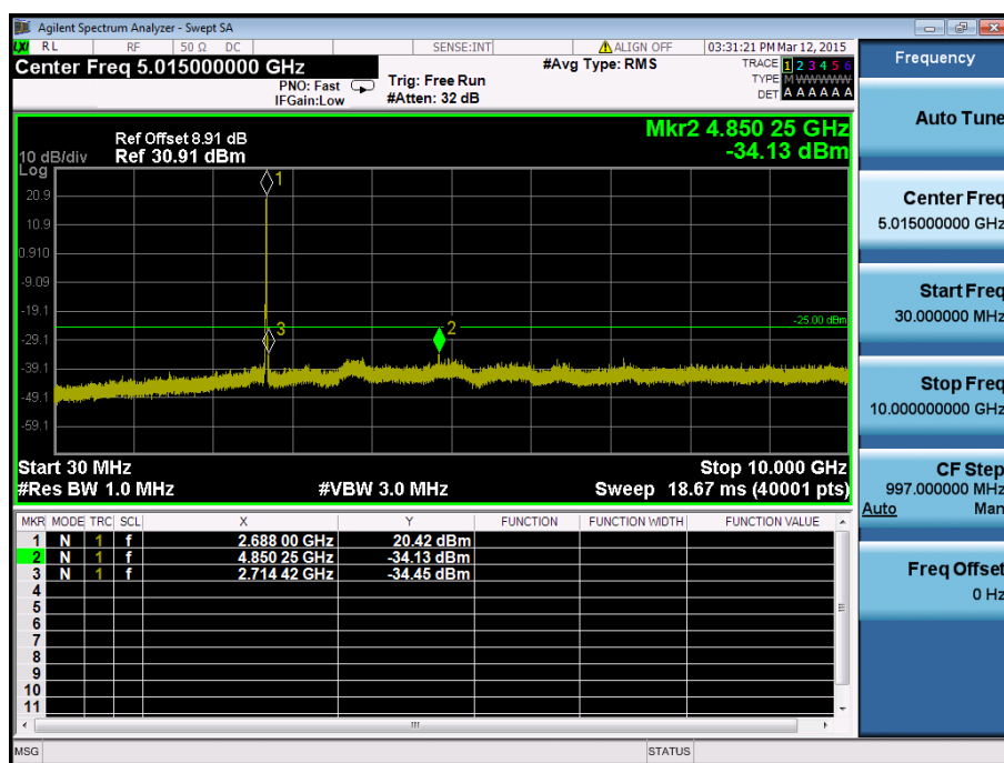
LTE Band 41 / 10MHz / 16QAM - RB Size/Offset (50/0) – High Channel
