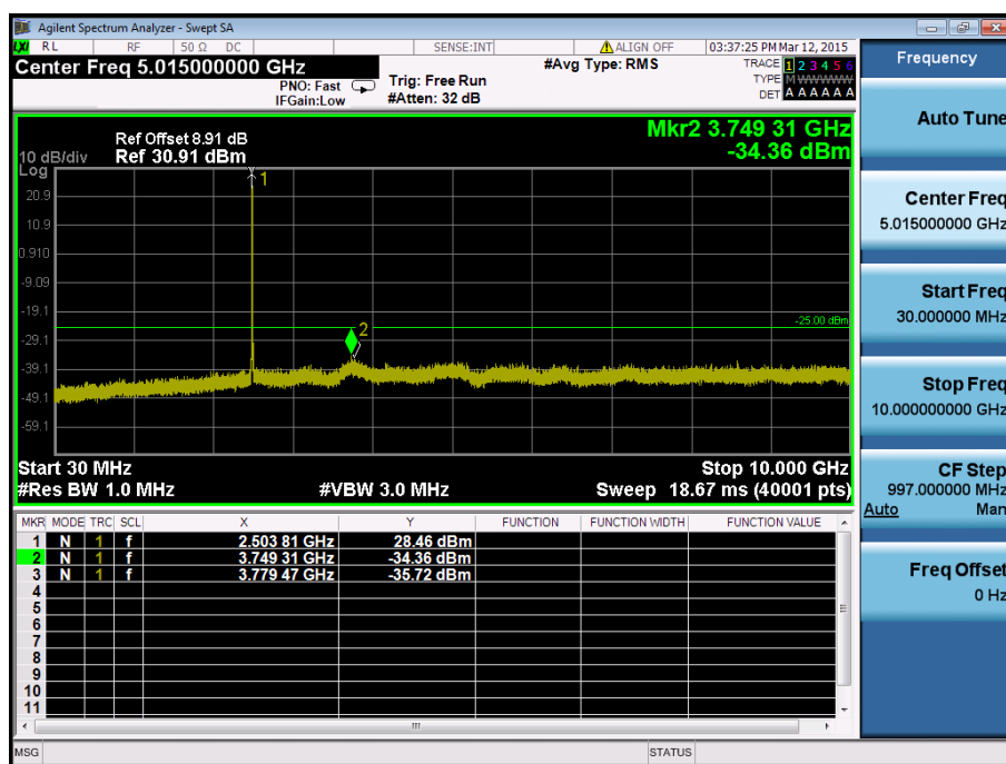
LTE Band 41 / 15MHz / 16QAM - RB Size/Offset (1/37) – Low Channel
