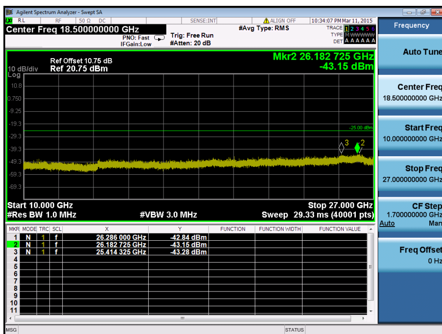
LTE Band 41 / 10MHz / QPSK - RB Size/Offset (1/0) – Low Channel
