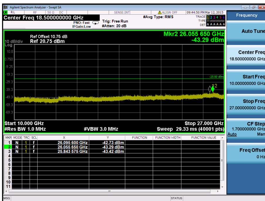
LTE Band 41 / 20MHz / 16QAM - RB Size/Offset (100/0) – High Channel
