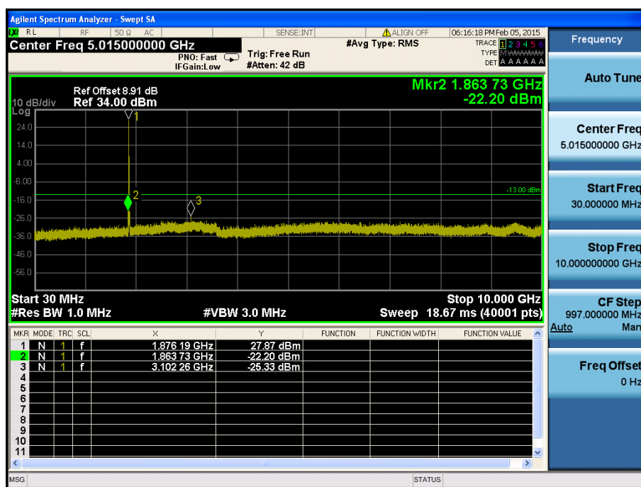
LTE Band 25 / 15MHz / QPSK - RB Size/Offset (1/0) – Mid Channel
