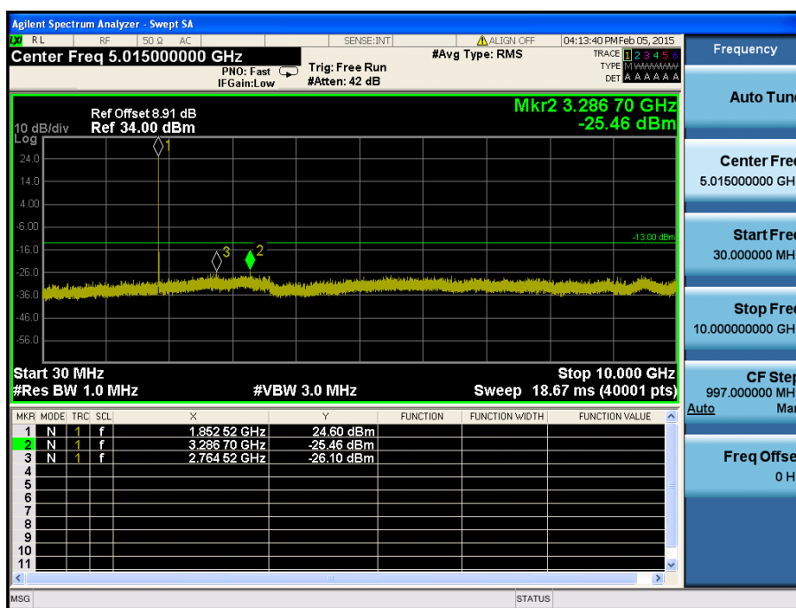
LTE Band 25 / 5MHz / QPSK - RB Size/Offset (12/0) – Low Channel
