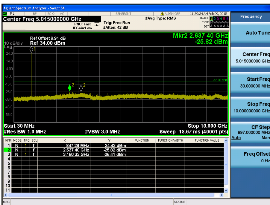
LTE Band 26 / 3MHz / 16QAM - RB Size/Offset (15/0) – High Channel
