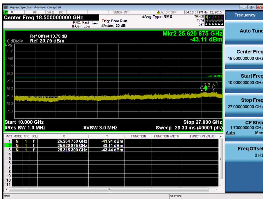
LTE Band 41 / 15MHz / 16QAM - RB Size/Offset (36/39) – Mid Channel
