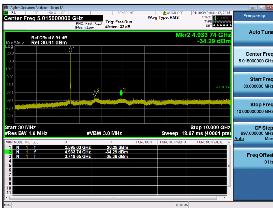
LTE Band 41 / 15MHz / 16QAM - RB Size/Offset (36/39) – Mid Channel
