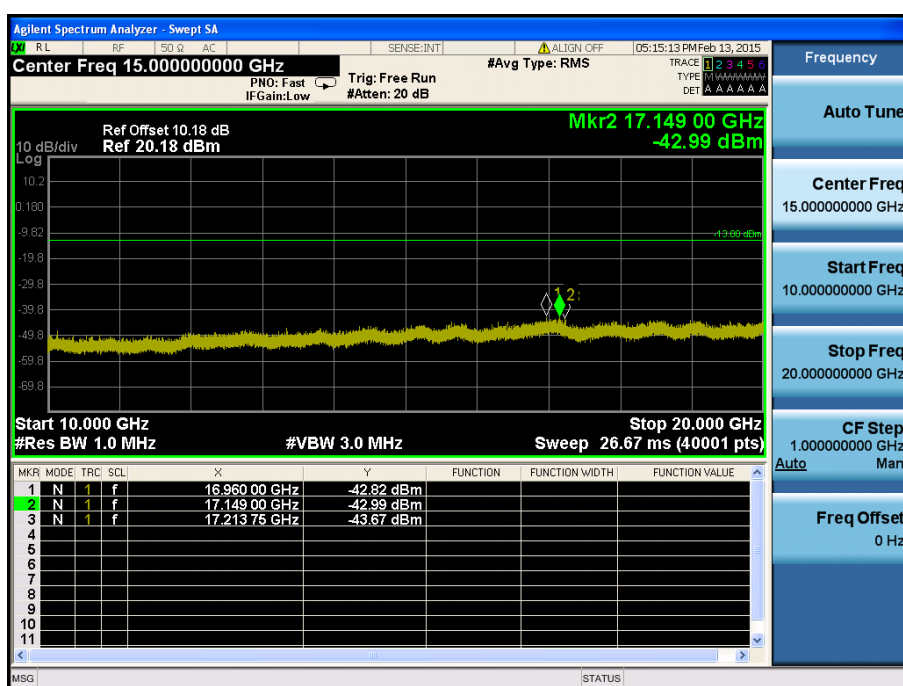
LTE Band 25 / 3MHz / 16QAM - RB Size/Offset (8/3) – Low Channel
