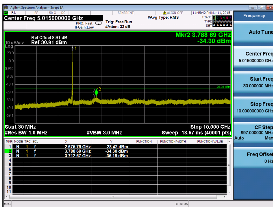
LTE Band 41 / 15MHz / QPSK - RB Size/Offset (1/0) – High Channel
