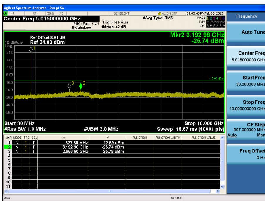
LTE Band 26 / 10MHz / QPSK - RB Size/Offset (25/0) – Low Channel
