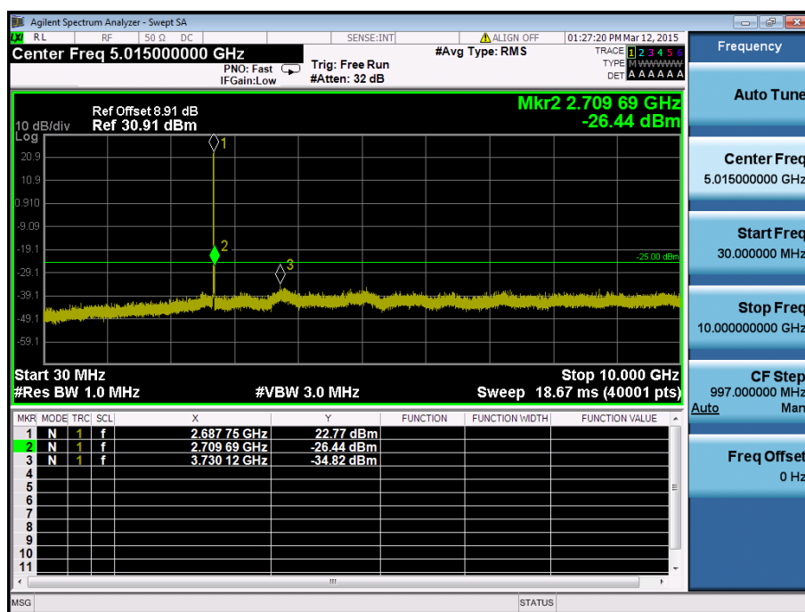
LTE Band 41 / 5MHz / 16QAM - RB Size/Offset (25/0) – High Channel
