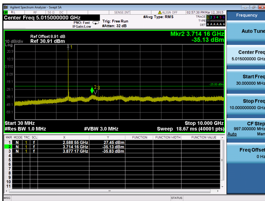
LTE Band 41 / 10MHz / 16QAM - RB Size/Offset (1/0) – Mid Channel
