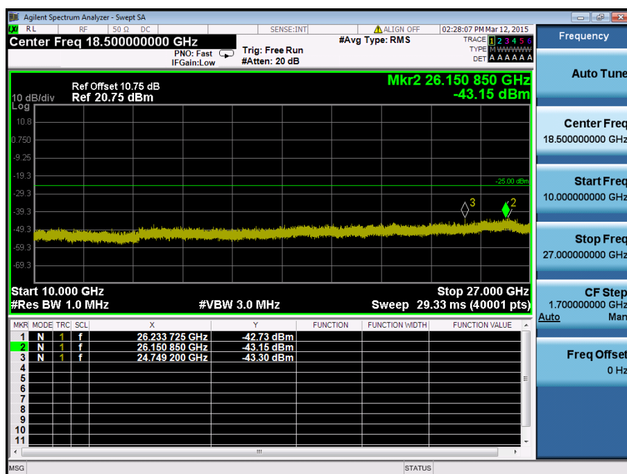
LTE Band 41 / 5MHz / 16QAM - RB Size/Offset (1/24) – Mid Channel
