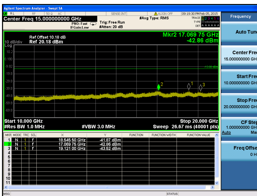
LTE Band 25 / 10MHz / 16QAM - RB Size/Offset (50/0) – Mid Channel
