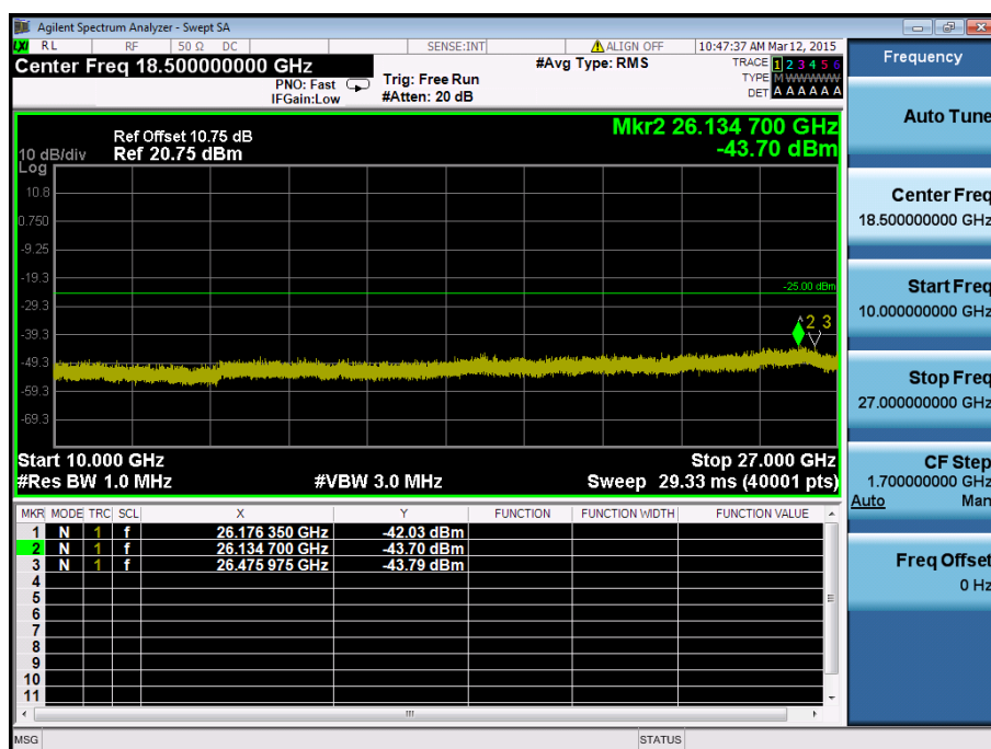
LTE Band 41 / 20MHz / QPSK - RB Size/Offset (50/25) – Mid Channel
