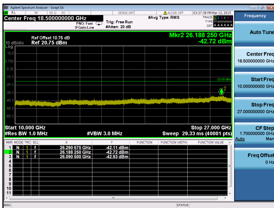
LTE Band 41 / 15MHz / 16QAM - RB Size/Offset (1/37) – Low Channel
