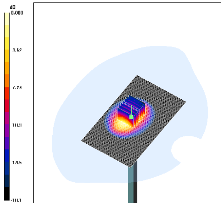
0 dB = 11.7mW/g
