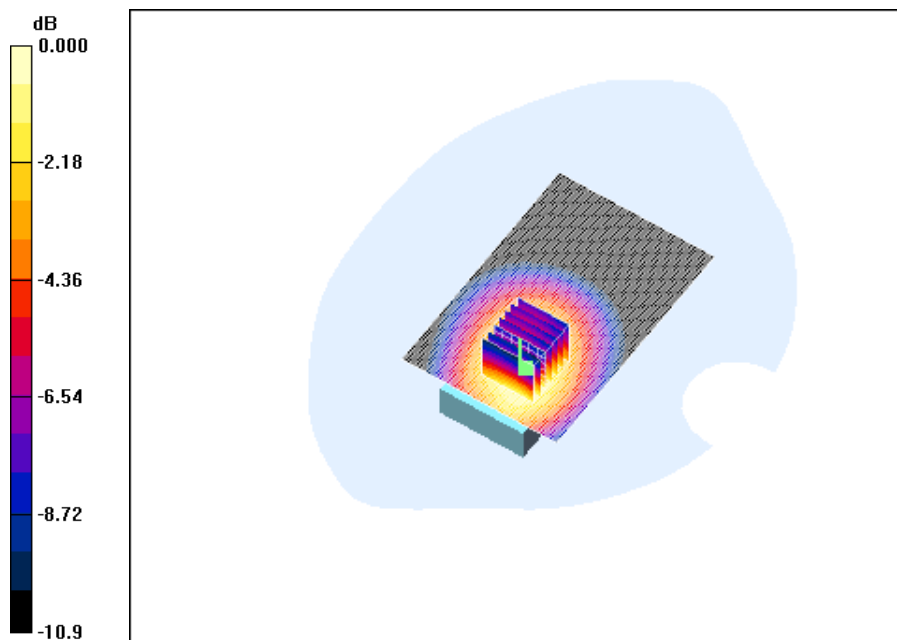
0 dB = 0.962mW/g
