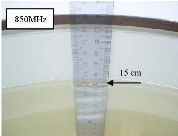
Fig.A-3a Photograph of the Tissue Simulant Liquid depth 15cm for Body Worn
