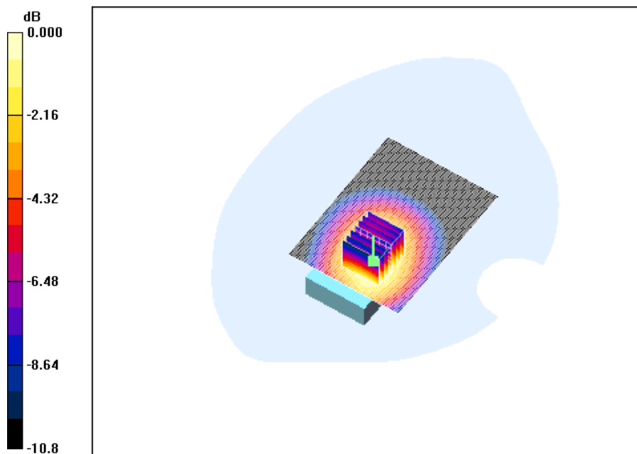
0 dB = 1.09mW/g
