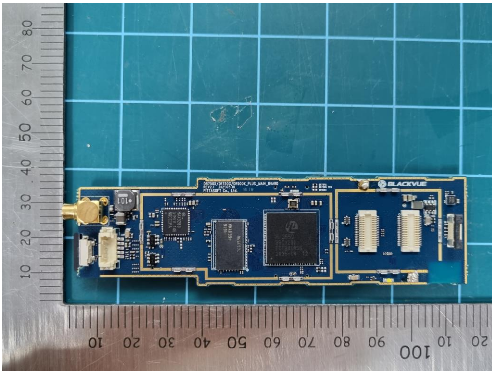
< Main PCB - Front - remove can >
