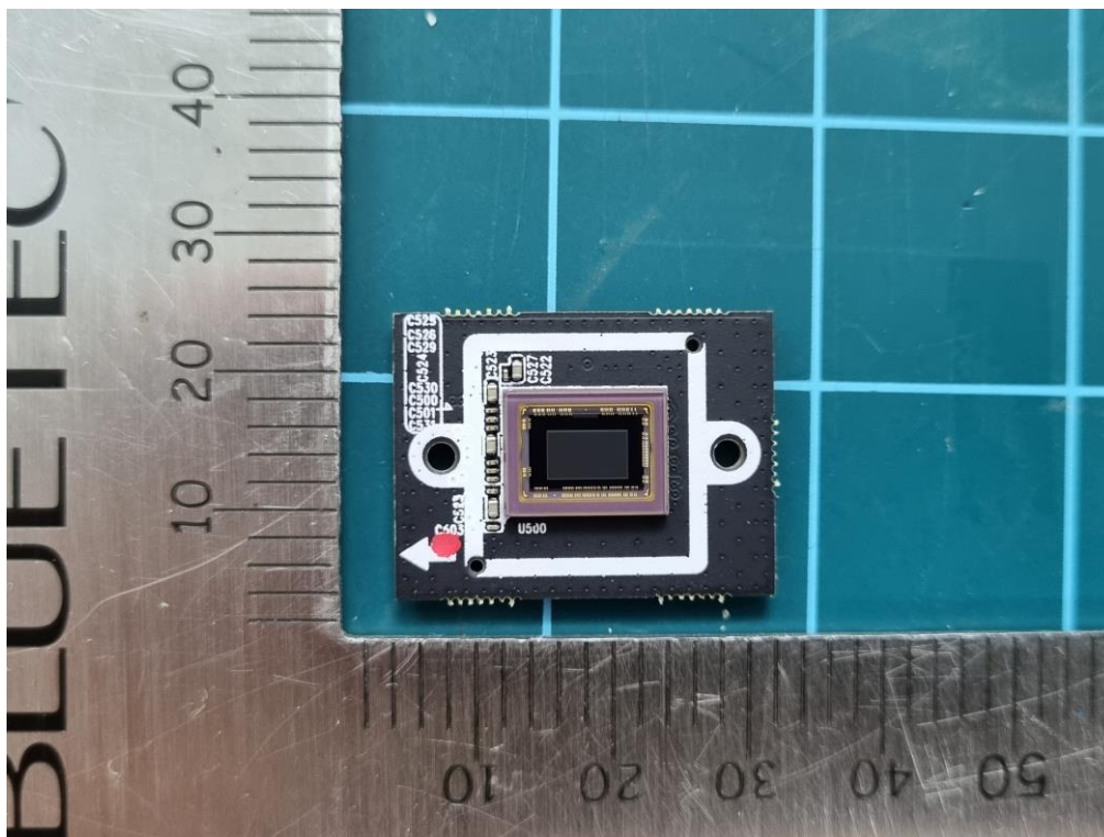
<Camera - Front>
