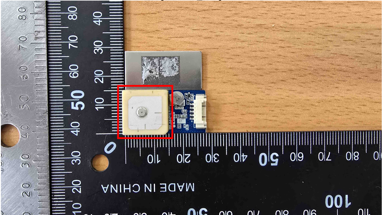
[Antenna_BLE & WLAN]
