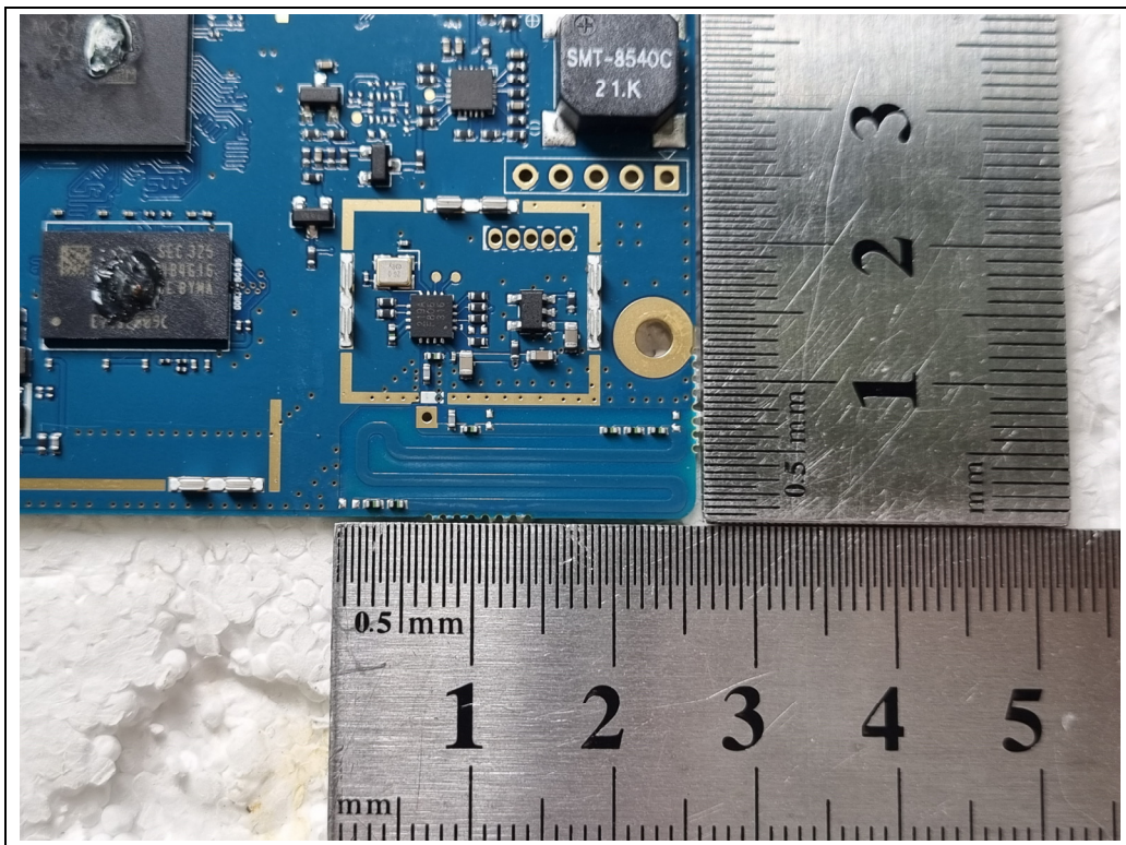
<400 MHz Band RX antenna>
