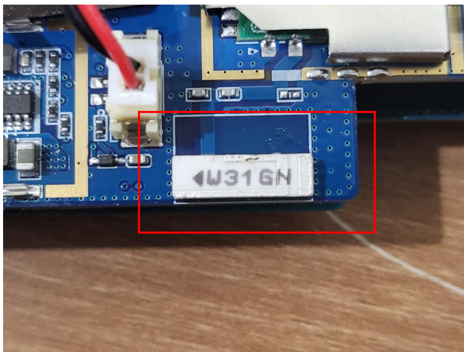
Bluetooth & WLAN Antenna
