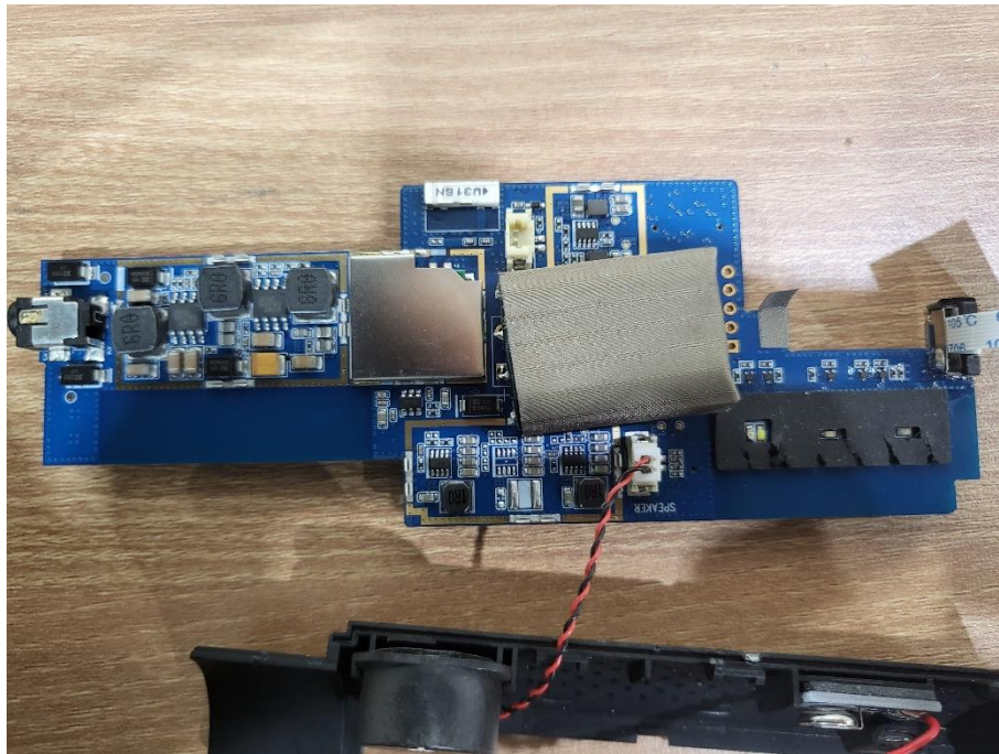
Power board (Remove shield) - Front Top
