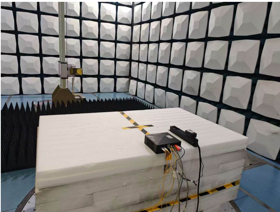
Radiated Emissions 1-18G Rear View M1
