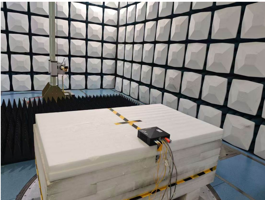
Radiated Emissions 18-26.5G Rear View M2
