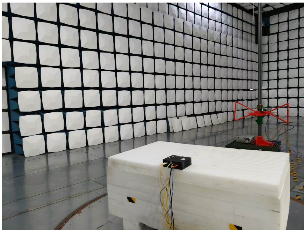
Radiated Emissions Below 1G side View M2
