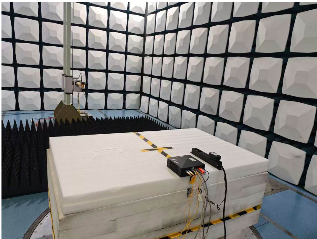
Radiated Emissions 26.5-30G Rear View M1
