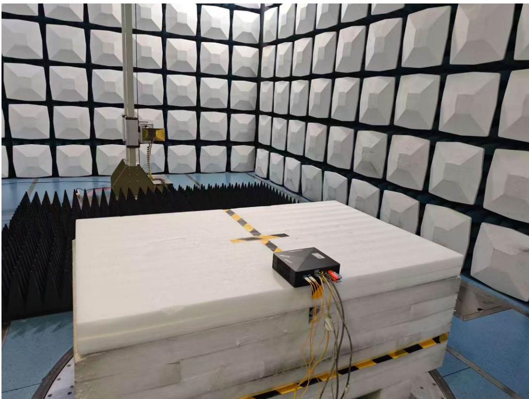
Radiated Emissions 1-18G Rear View M2
