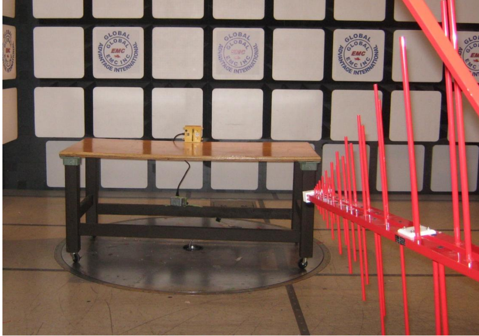
Radiated emissions testing (EUT tested in plastic enclosure)
