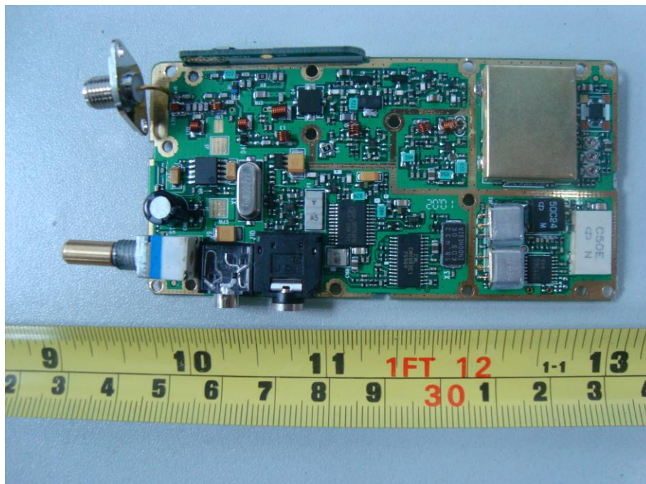
EUT – Main Board Bottom Components View 1
