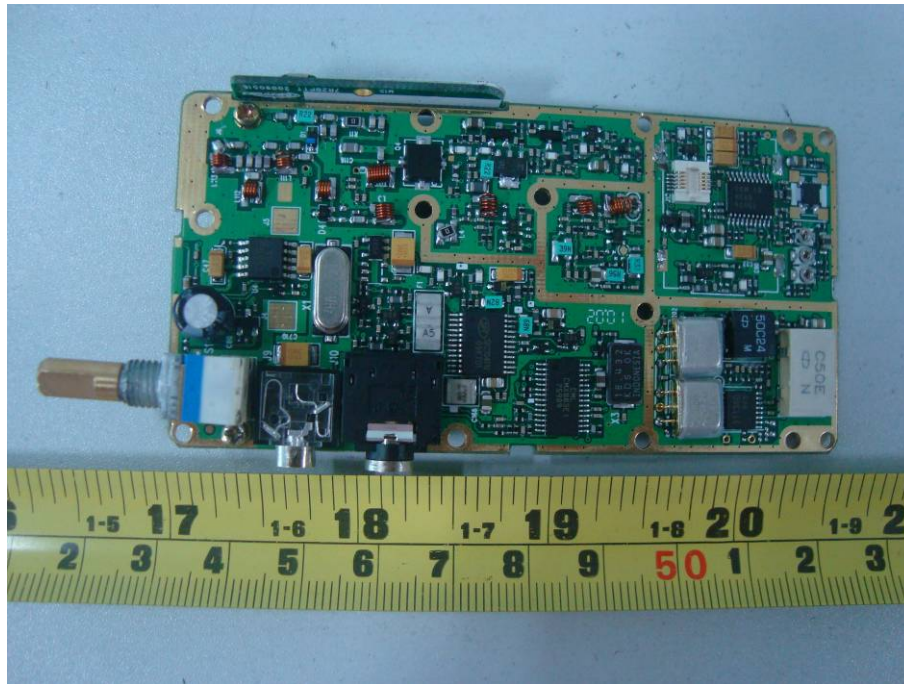
EUT – Main Board Bottom Components View 2
