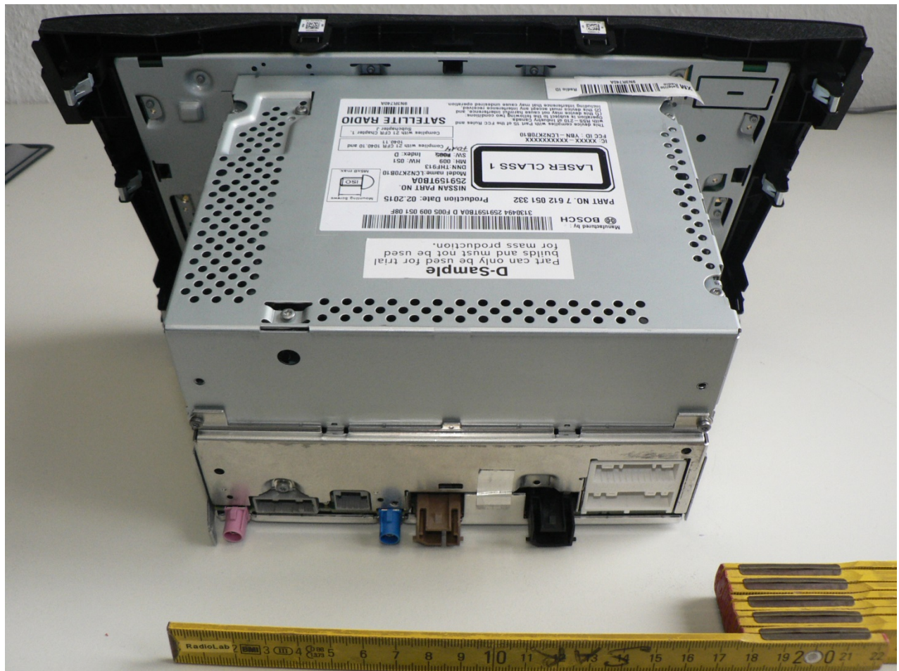
1.1.2. Photograph: rear view
