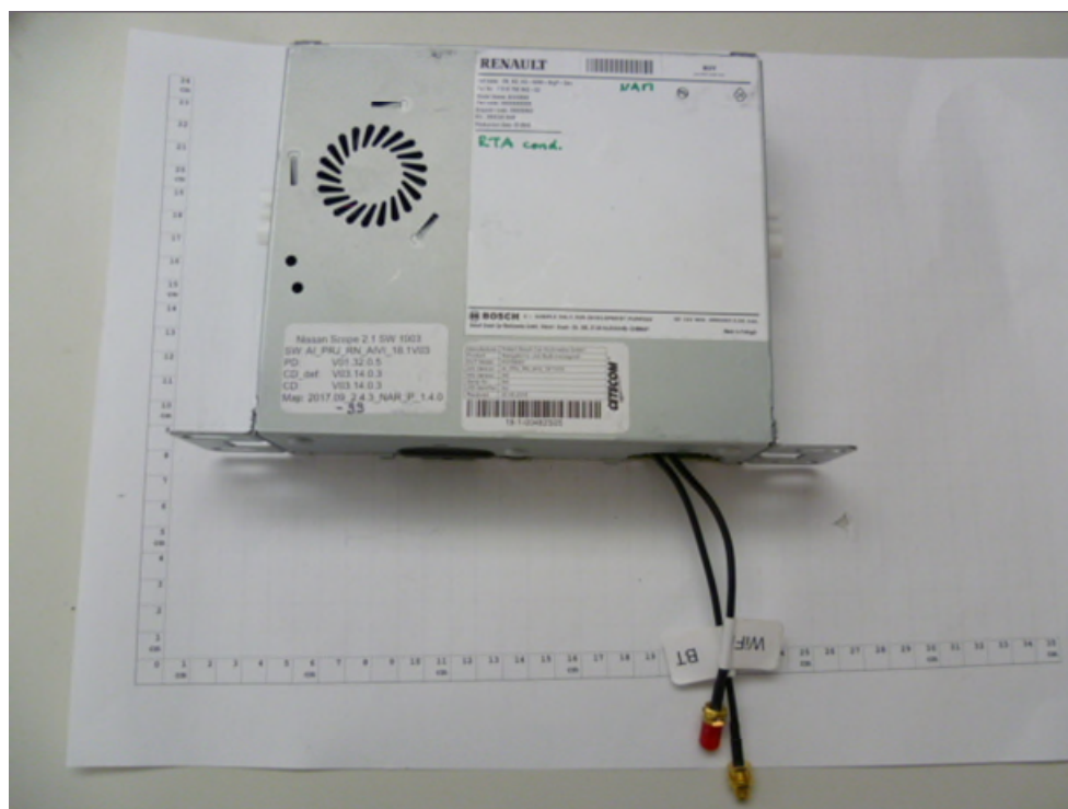
Photograph 7: EUT conducted sample
