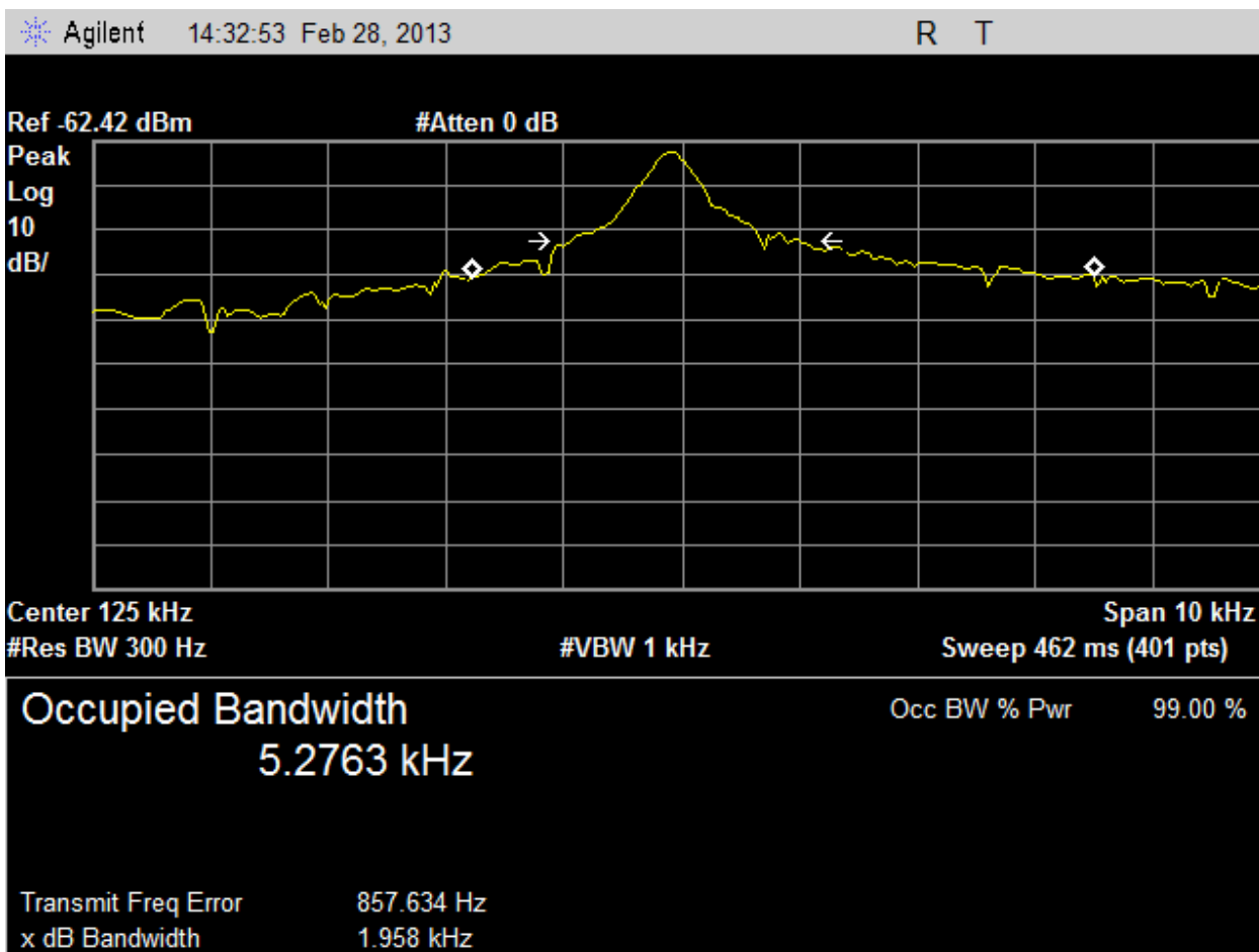
Plot 2 – 20dB BW FSK Modulation & 99% Occupied BW (For IC Only)
