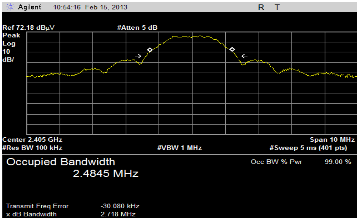
Plot 2 – 20dB BW FSK Modulation & 99% Occupied BW (For IC Only)
