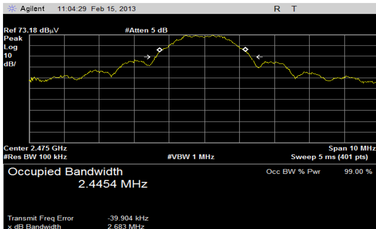
Plot 4 – 20dB BW FSK Modulation & 99% Occupied BW (For IC Only)
