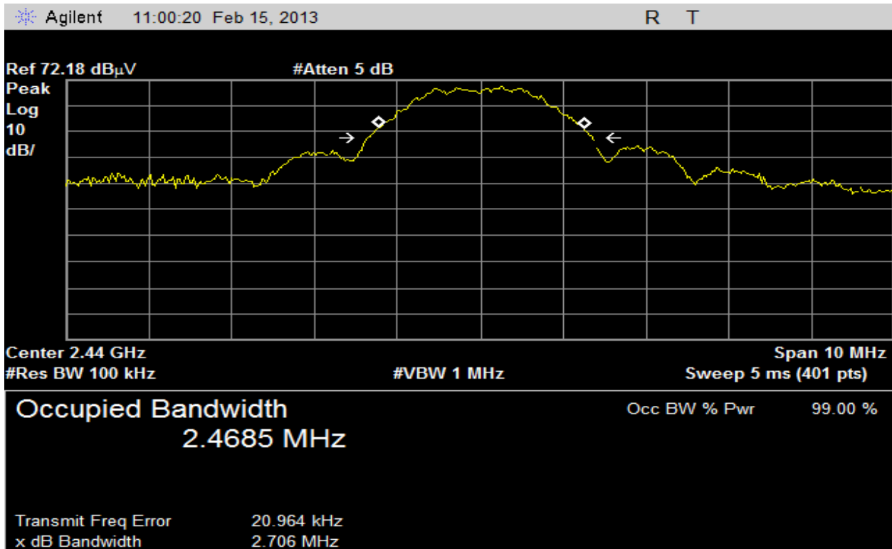
Plot 3 – 20dB BW FSK Modulation & 99% Occupied BW (For IC Only)
