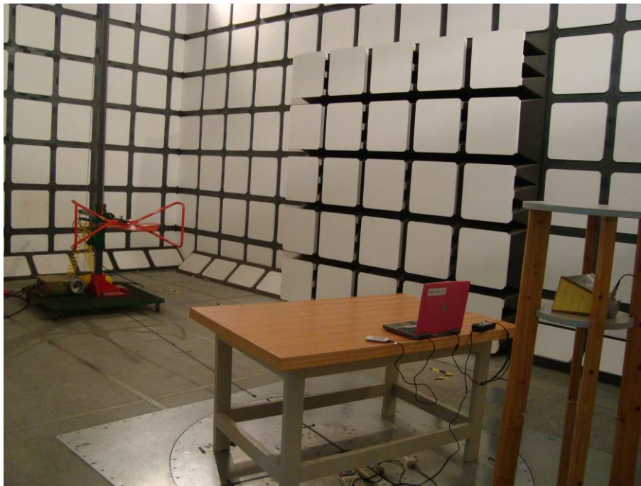
Below 1 GHz: Radiated Emissions - Rear View (PC Charging & Transmitting Mode)
