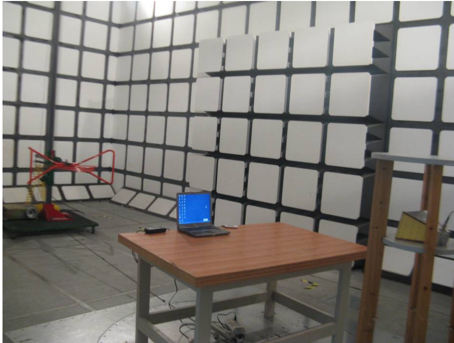
Below 1 GHz: Radiated Emissions - Front View (PC Charging & Transmitting Mode)
