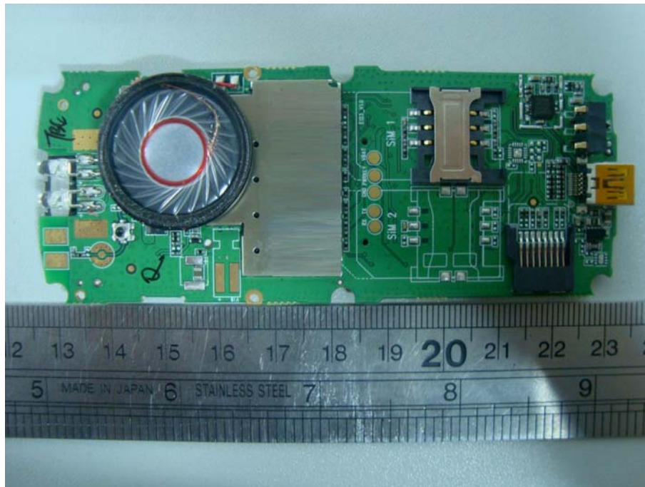
EUT – Main Board Top without Screen View
