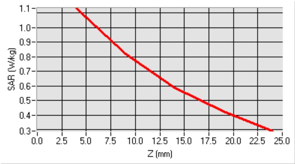
SAR, Z Axis Scan (X = -26, Y = -17)
