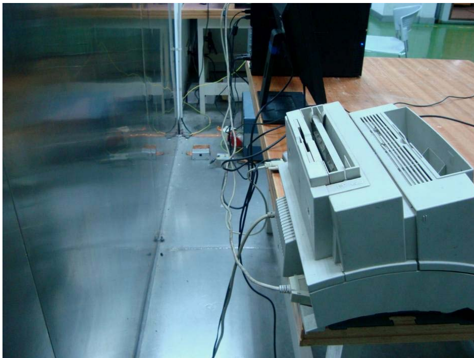
AC Line Conducted Emissions - Side View (Downloading Mode)
