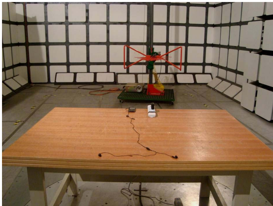
Spurious Radiated Emissions - Rear View (Media Playing & Charging Mode)
