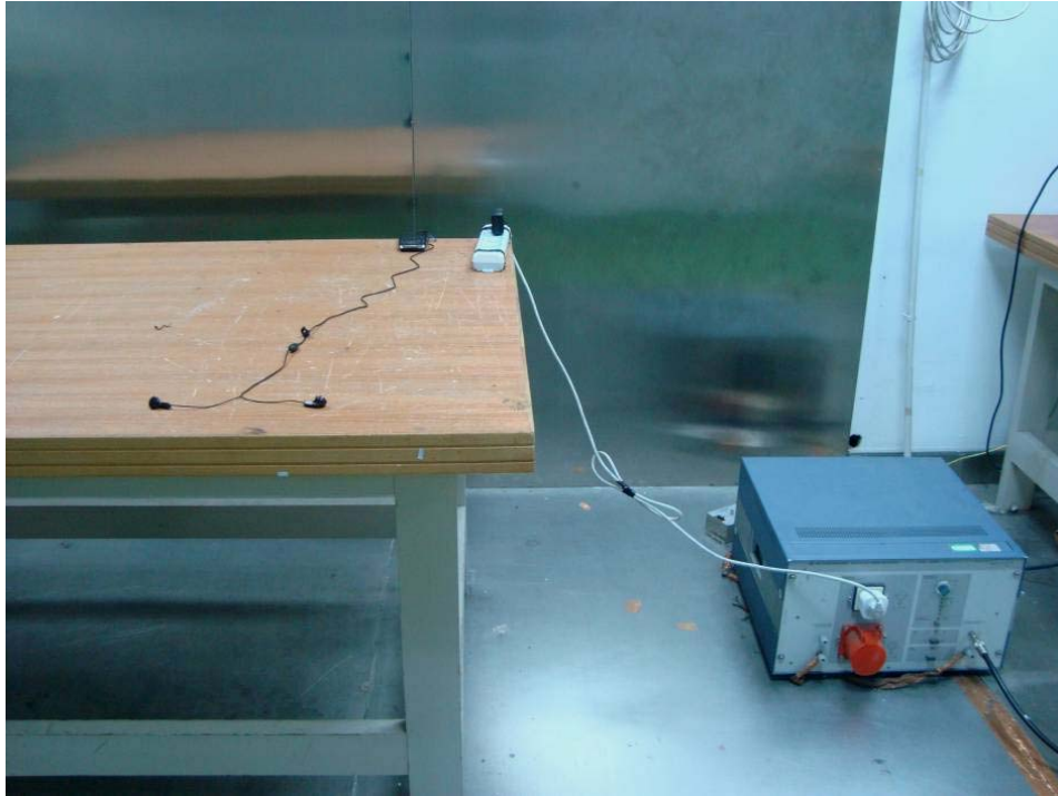
AC Line Conducted Emissions - Side View (Media Playing & Charging Mode)
