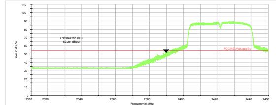
802.11n HT40 -Channel 3 Average
