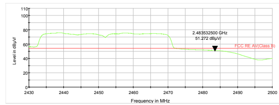
802.11n HT40 -Channel 9 Average
