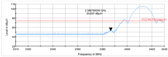
802.11b-Channel 1 Peak
