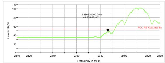
802.11b-Channel 1 Average
