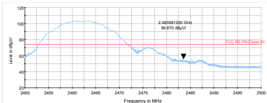
802.11b-Channel 11 Peak
