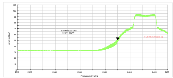
802.11g-Channel 1 Average
