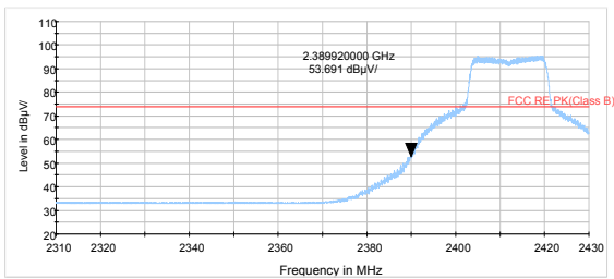
802.11g-Channel 1 Peak
