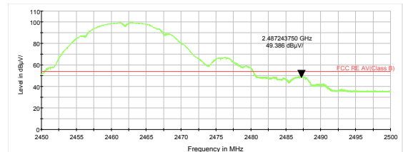
802.11b-Channel 11 Average
