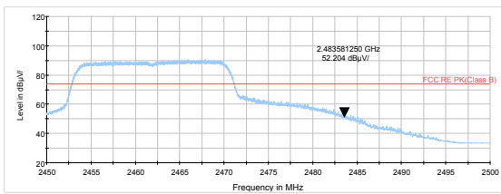
802.11g-Channel 11 Peak
