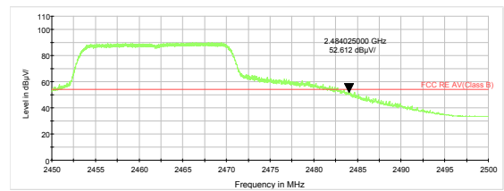
802.11g-Channel 11 Average
