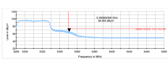
802.11n HT40-Channel 62: Peak
