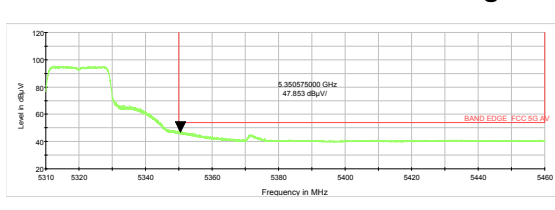
802.11n HT20-Channel 64: Average
