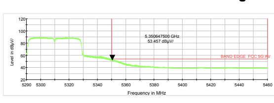
802.11n HT40-Channel 62: Average
