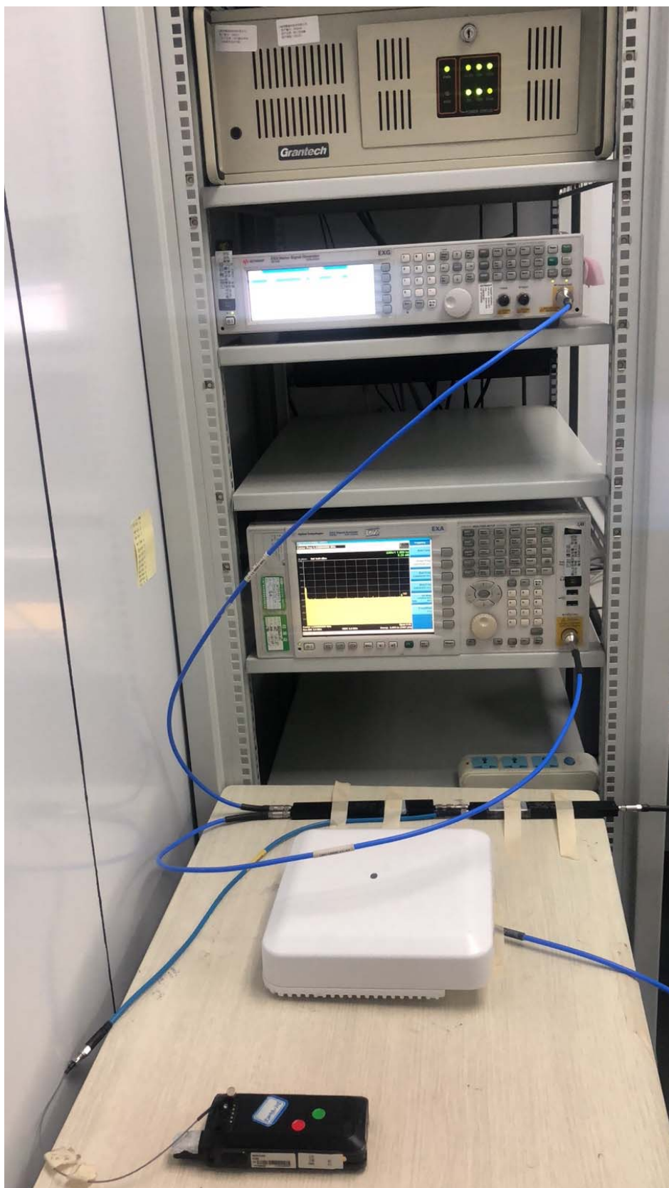
Picture 1 Test Setup
