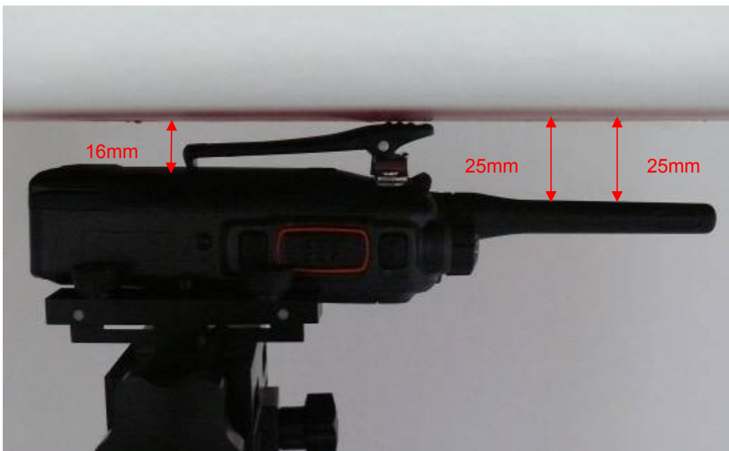
Picture 5: Body-worn, The EUT display towards ground, Belt clip attach the Phantom, the distance from EUT Antenna to the bottom of the Phantom is 25mm
