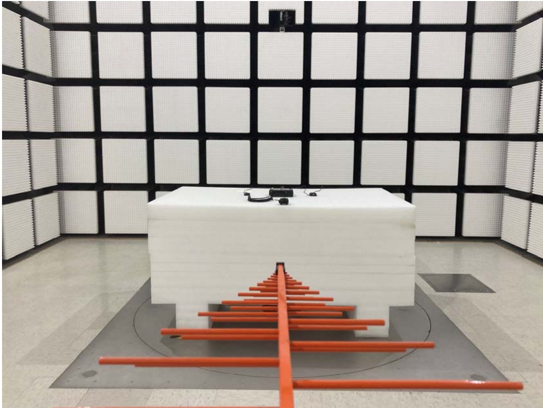
Radiated Emission Below 1GHz View- Model: MD622 VHF
