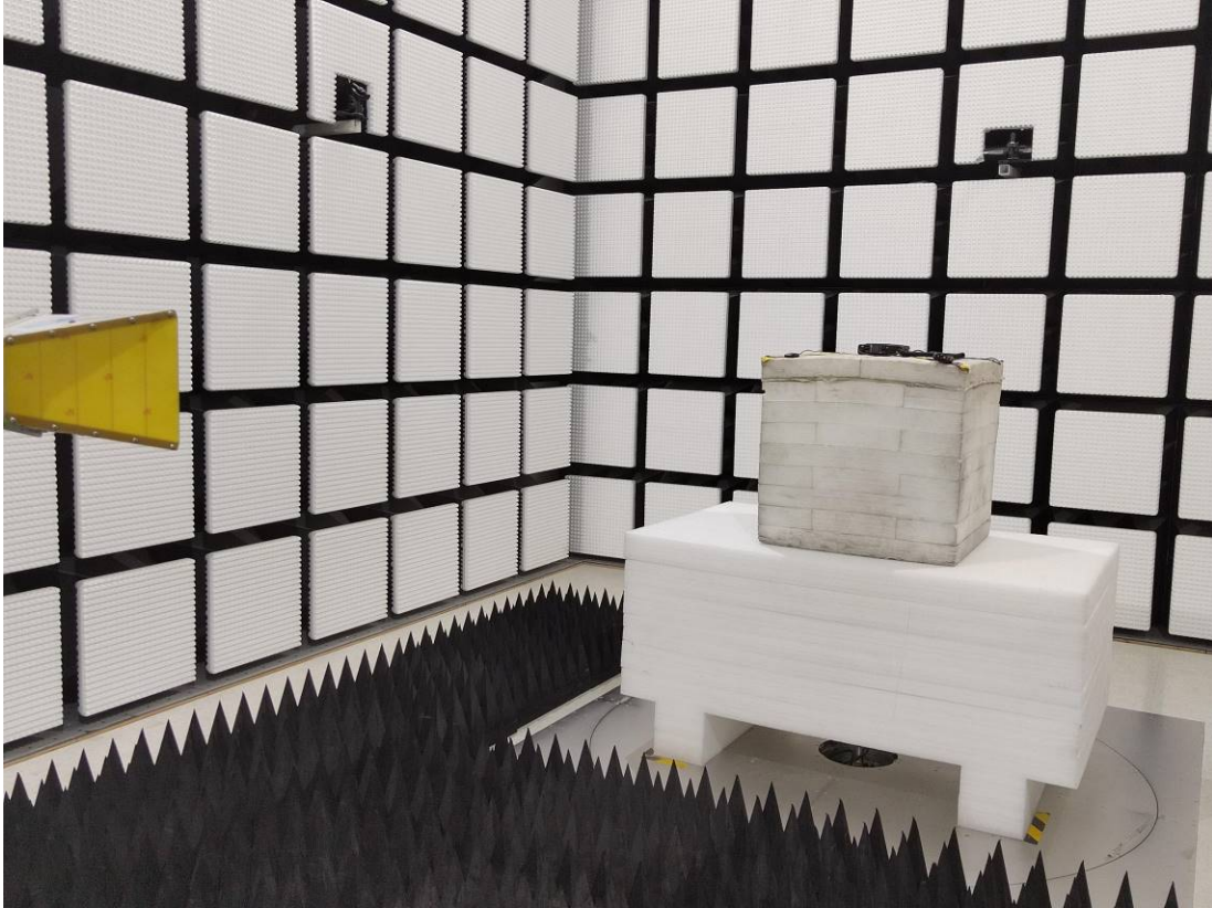
Radiated Emission Above 1GHz View-Model: HM652 U1
