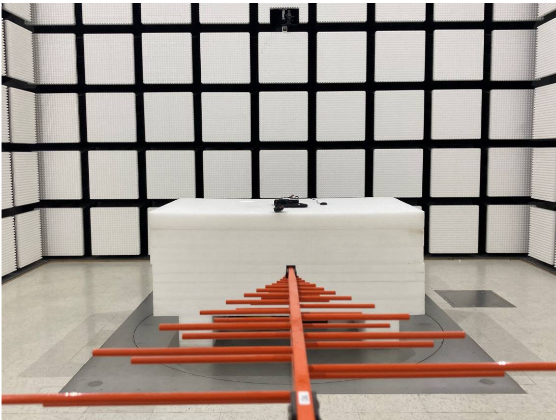
Radiated Emission Below 1GHz View-Model: HM652 U1
