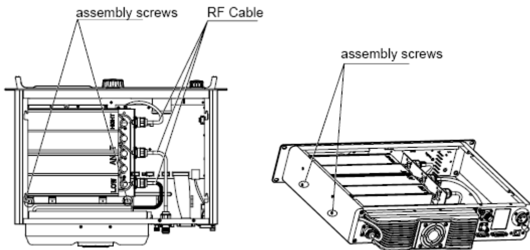
Duplexer with Front Side Facing Upwards
