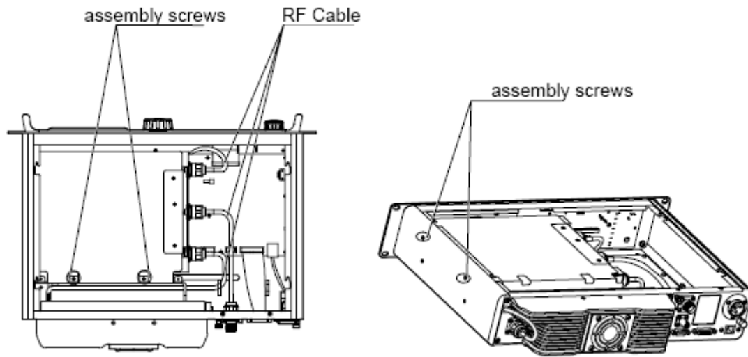
Duplexer with Front Side Facing Downwards
