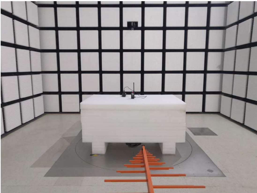
Radiated Emission Below 1GHz View- USB Mode
