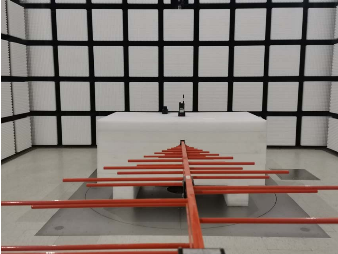
Radiated Emission Below 1GHz View-USB Power Mode
