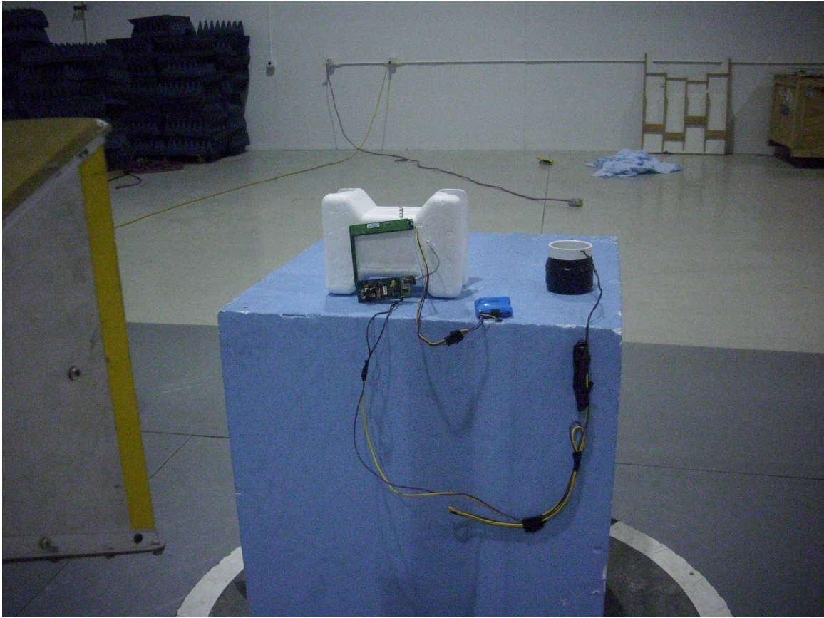
Radiated Spurious Emissions Above 1GHz
