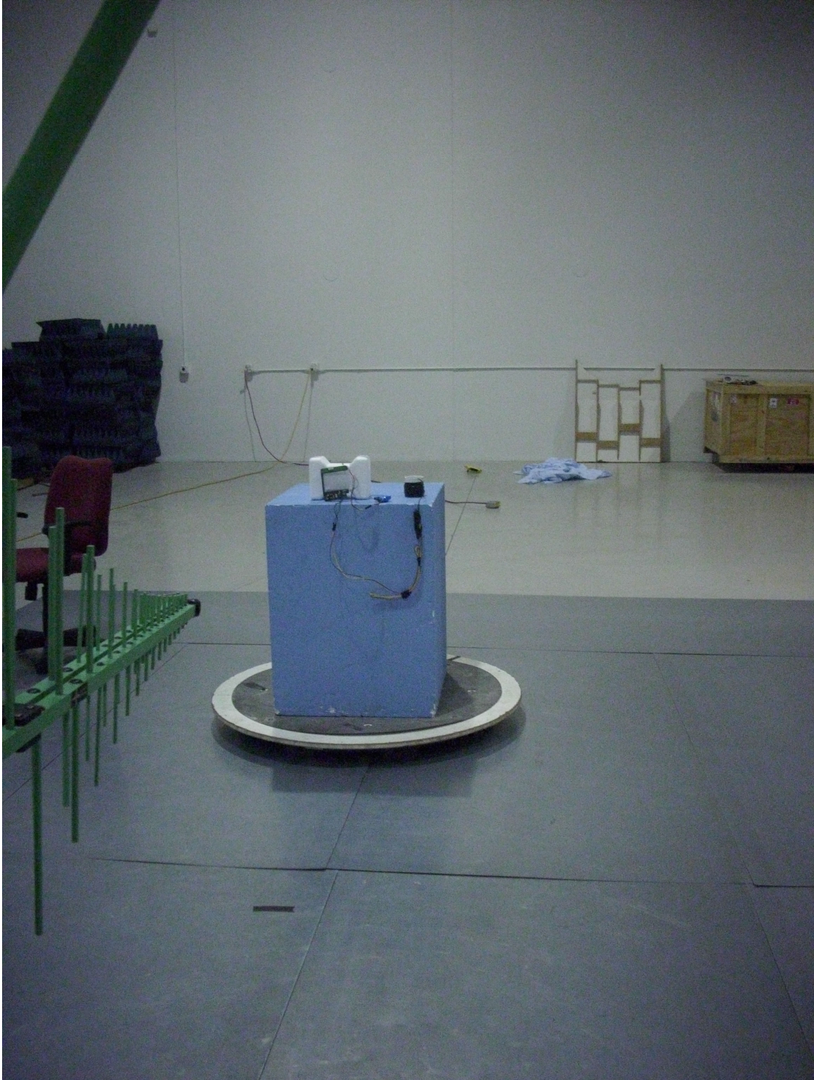
Radiated Spurious Emissions 30-1000MHz
