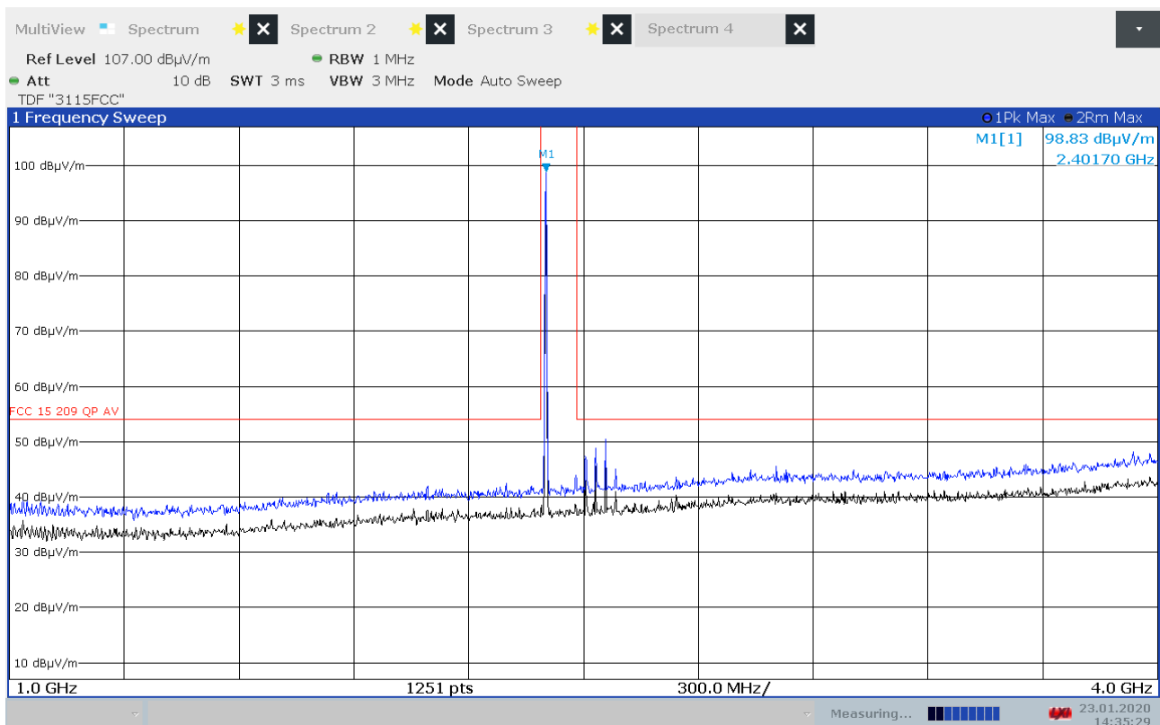
Radiated Emissions, 1000 -4000MHz, 2402MHz, GFSK, VP
