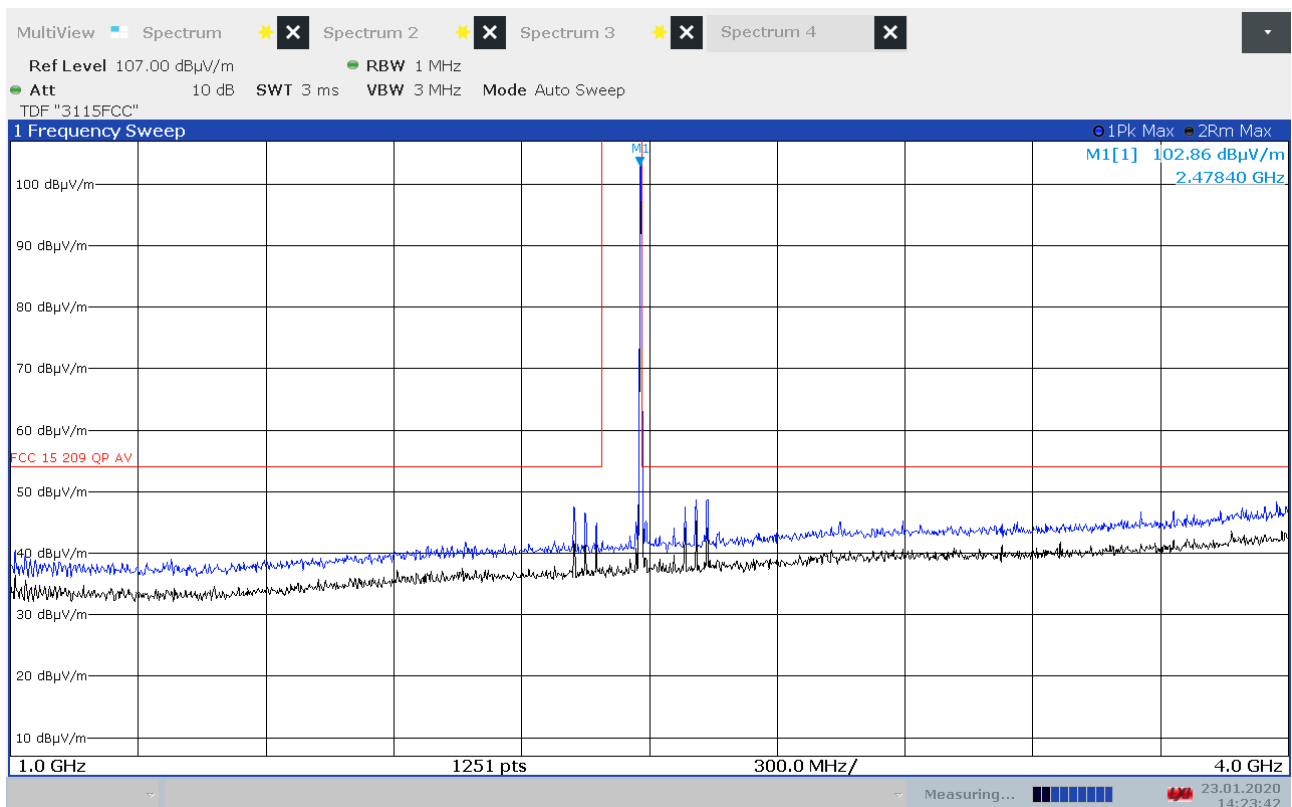
Radiated Emissions, 1000 -4000MHz, 2480MHz, GFSK, VP
