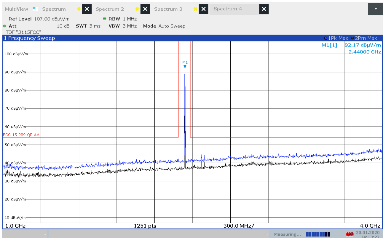
Radiated Emissions, 1000 -4000MHz, 2440MHz, GFSK, HP
