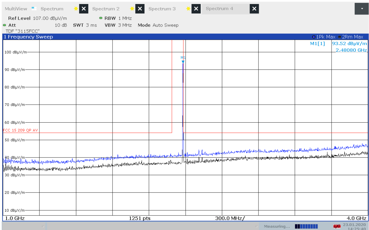
Radiated Emissions, 1000 -4000MHz, 2480MHz, GFSK, HP
