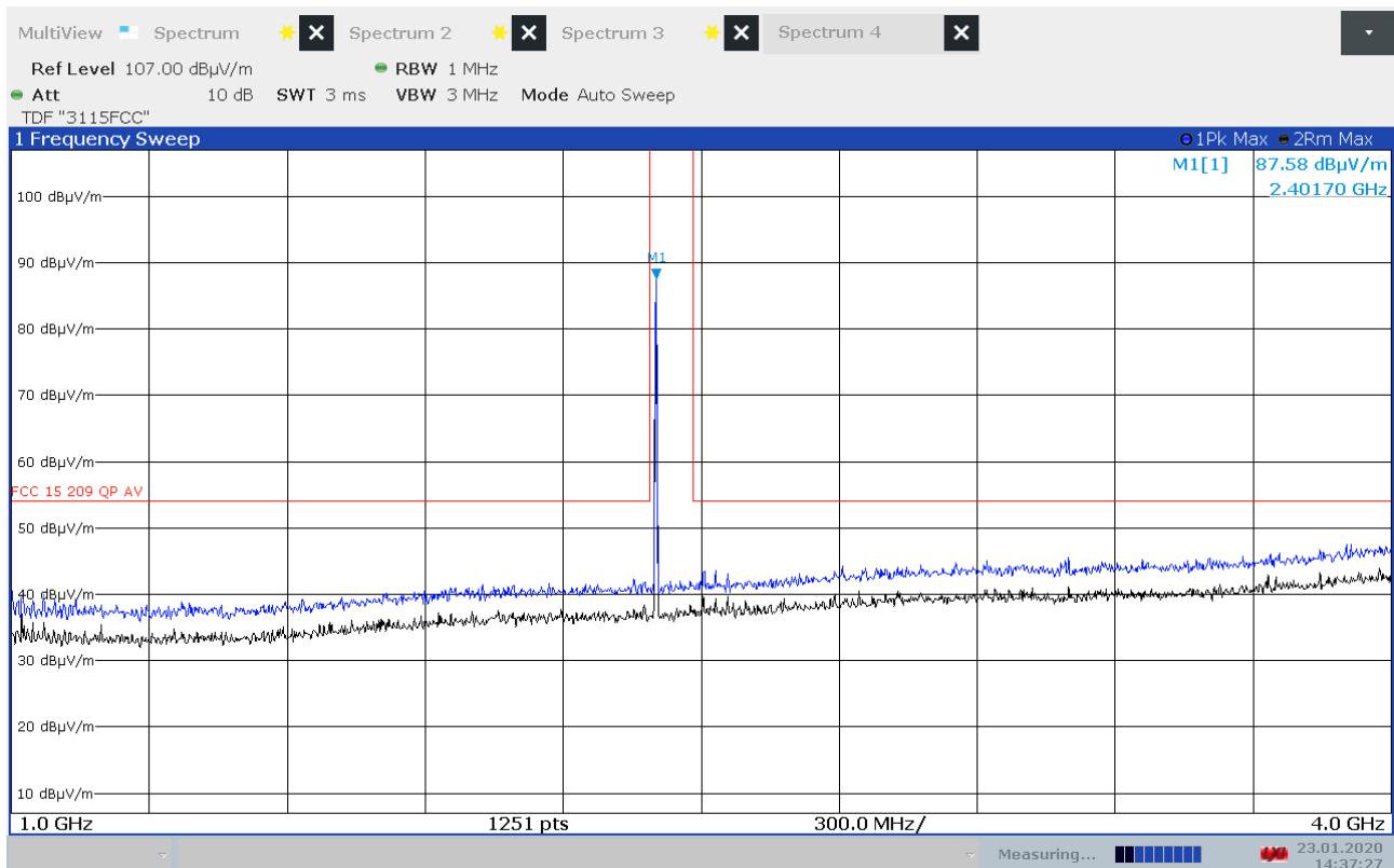
Radiated Emissions, 1000 -4000MHz, 2402MHz, GFSK, HP
