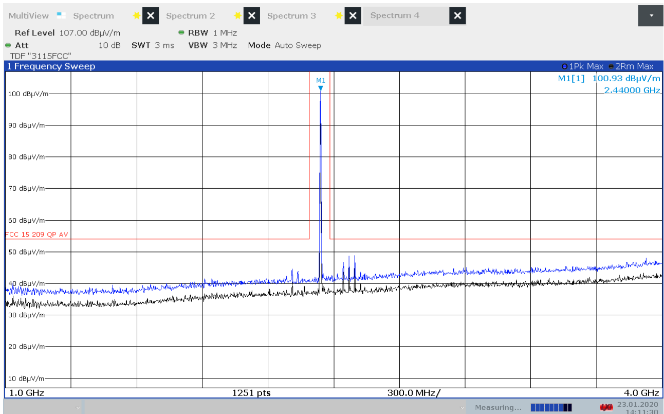
Radiated Emissions, 1000 -4000MHz, 2440MHz, GFSK, VP
