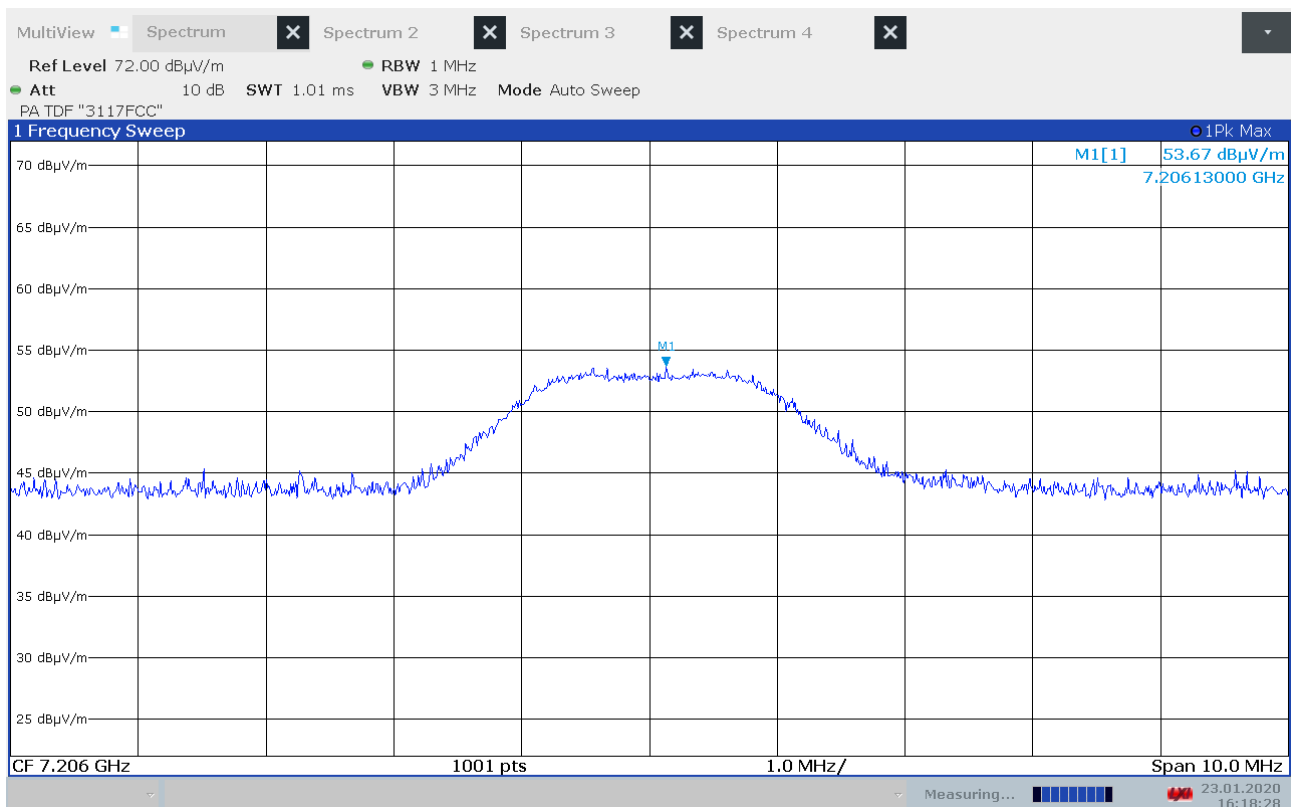
Maximum Radiated Emissions, 7206MHz, 2402MHz, GFSK
