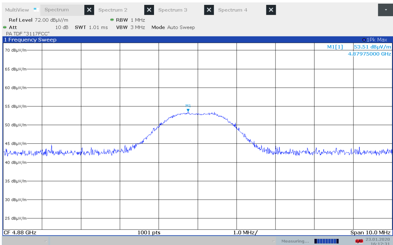
Maximum Radiated Emissions, 4880MHz, 2440MHz, GFSK
