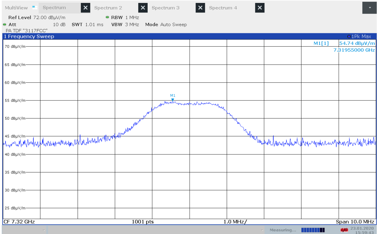
Maximum Radiated Emissions, 7320MHz, 2440MHz, GFSK
