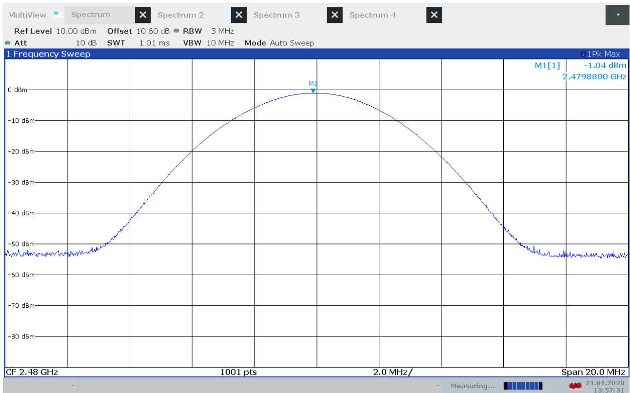
Output Power, 2480 MHz, 8-DPSK
