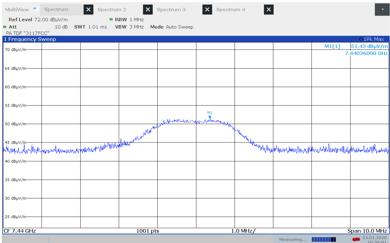
Maximum Radiated Emissions, 7440MHz, 2480MHz, GFSK
