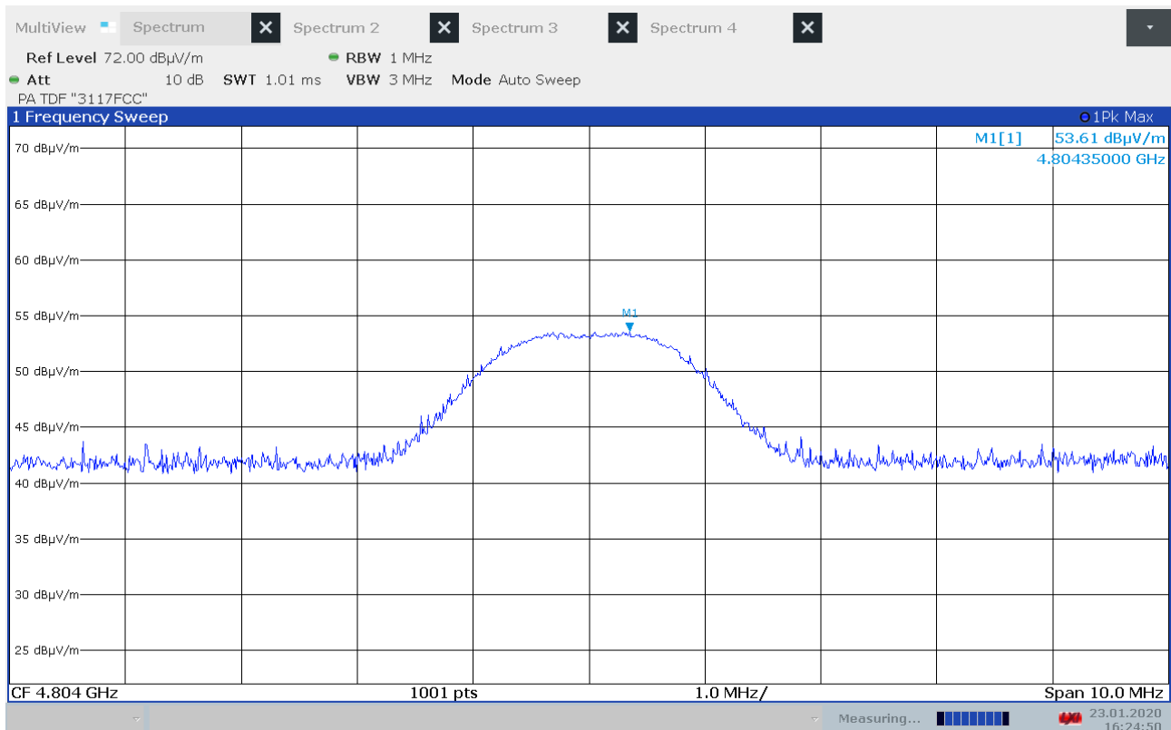
Maximum Radiated Emissions, 4804MHz, 2402MHz, GFSK
