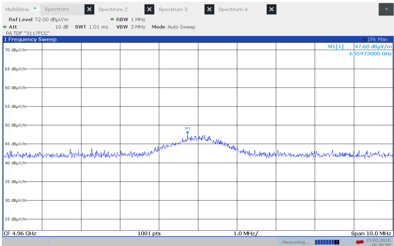
Maximum Radiated Emissions, 4960MHz, 2480MHz, GFSK
