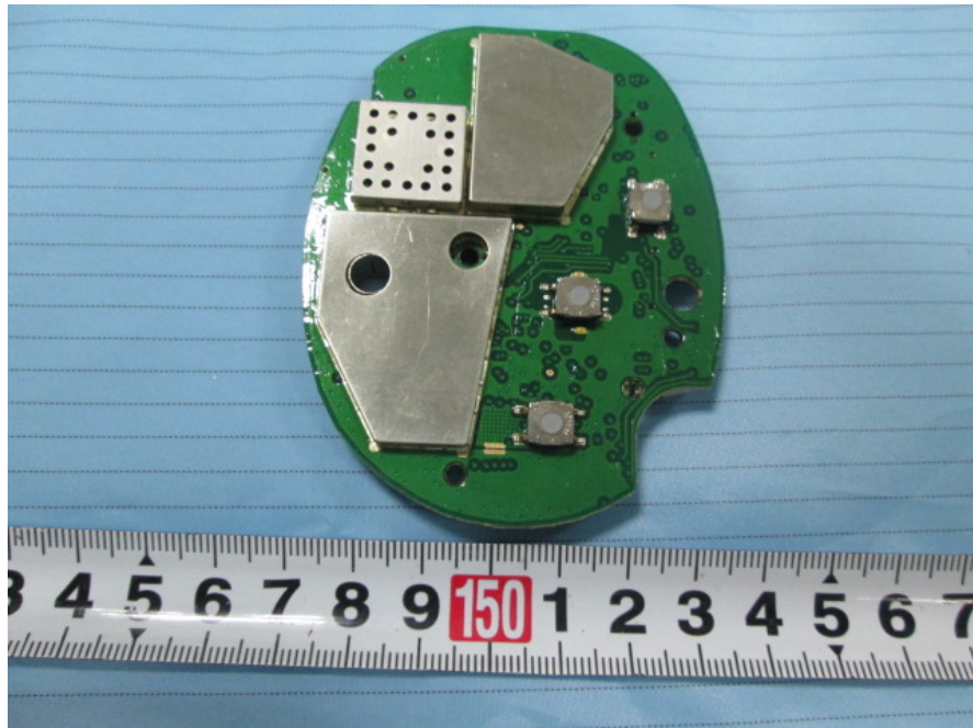
EUT –Right Main Board #1 View
