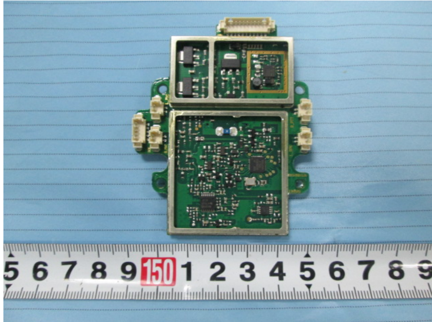
EUT –Left Main Board #3 View
