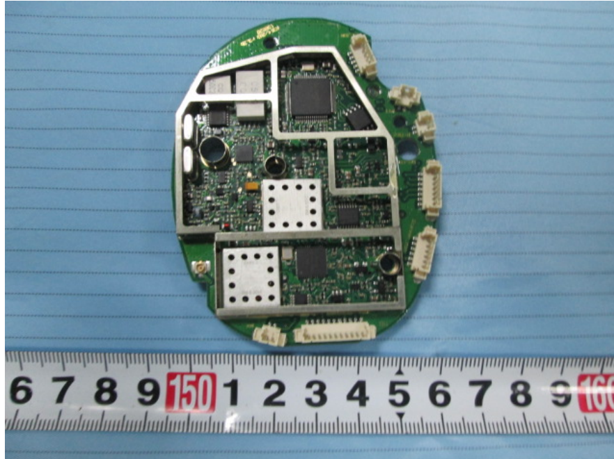
EUT –Right Main Board #4 View
