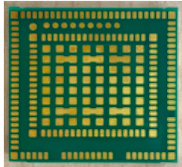
Back side of the module
