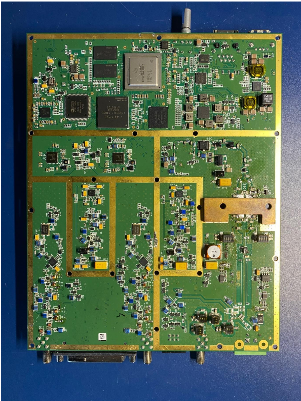
KA-500e Main board (bottom view)
