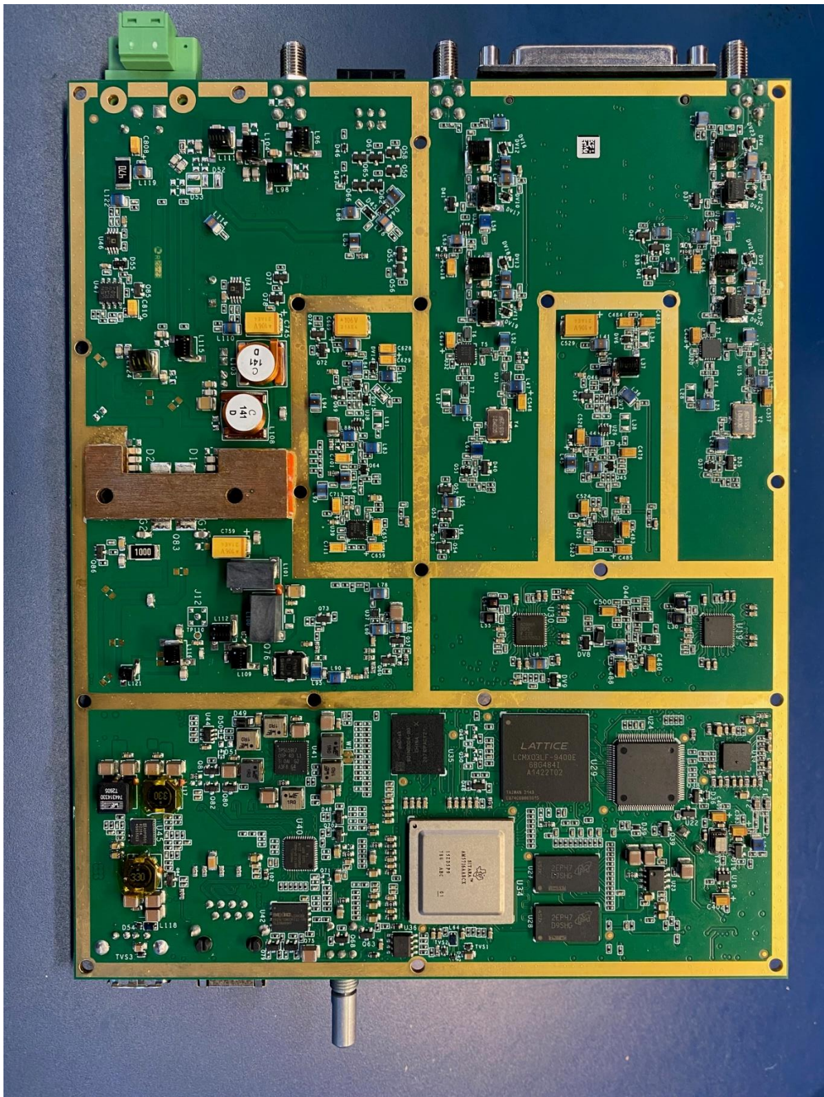
KA-080e Main board (bottom view)
