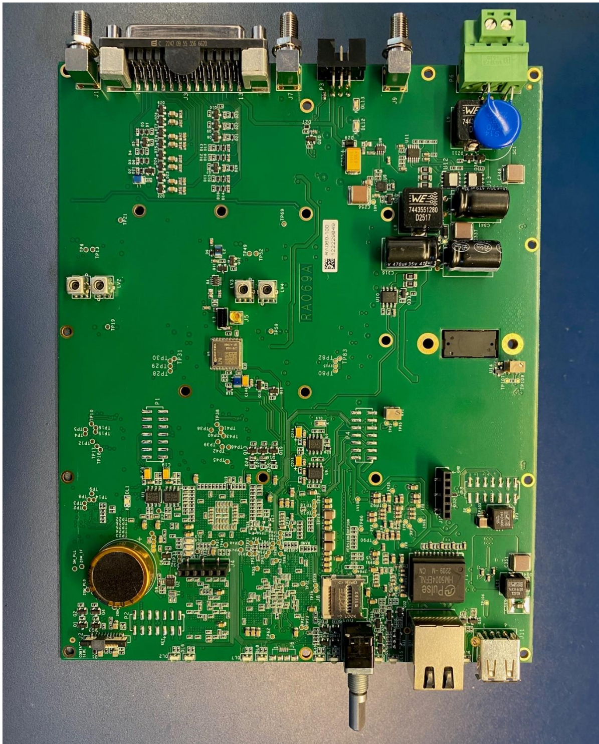
KA-080e Main board (top view)
