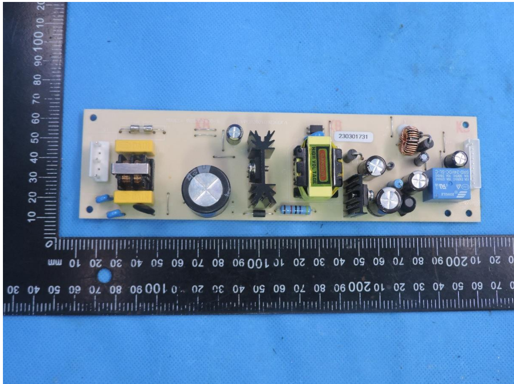
Photo 16 (Power board model: P037D240O-9)
