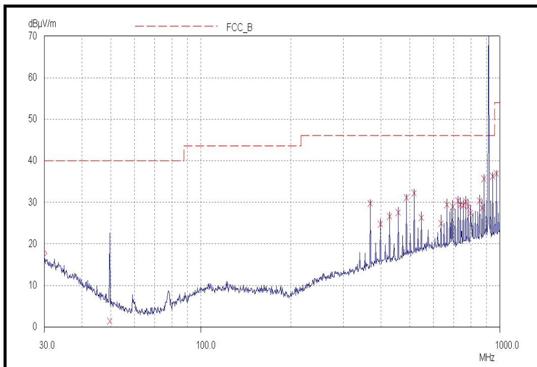
Radiated spurious emissions 30 MHz to 1 GHz
