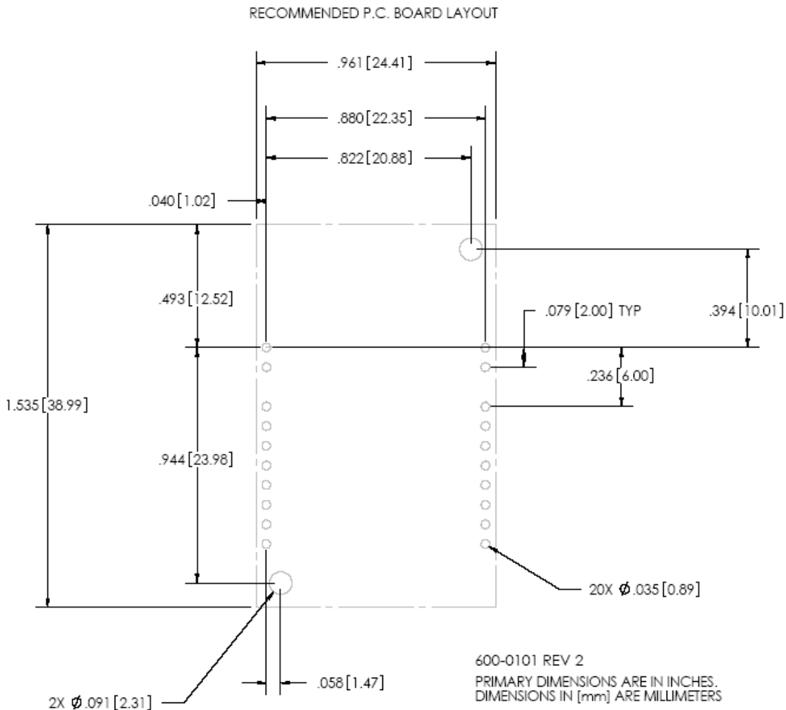
Figure 14 M2511 Mote Footprint
