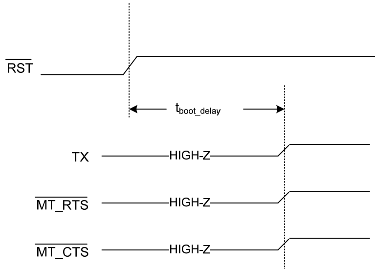
Figure 8 Power-on Sequence (see section 7.1 for value of t_{\text{boot\_delay}} )
