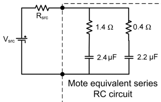
Figure 4 M2511 Equivalent Series RC Circuit
