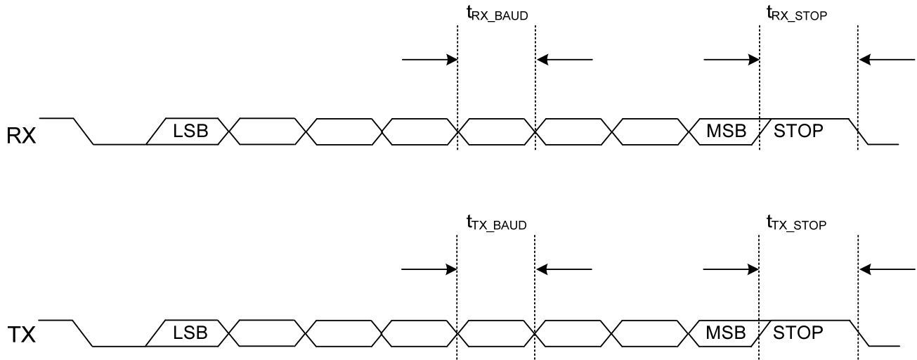
Figure 9 Byte-level Timing
