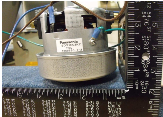
Motor view side
